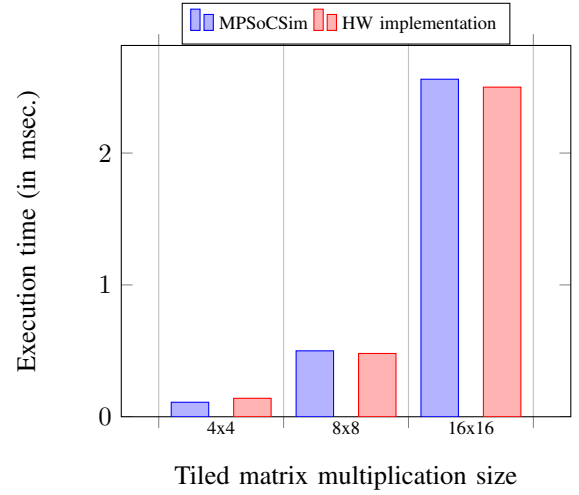
Fig. 3. Comparison between MPSoCSim and the HW implementation [1]
