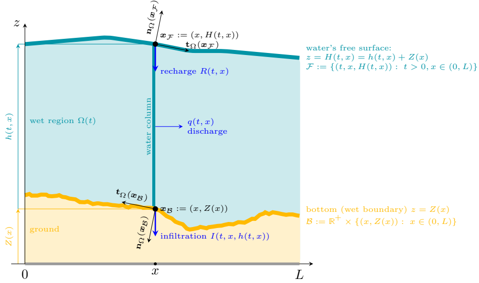
FIGURE 1. Schematic setting of the model, color coded with a water color, ground color, and flow color, where by “flow” we mean any source of variation of the water quantity, including the boundary fluxes (indicated with arrows, but in fact scalar quantities).
