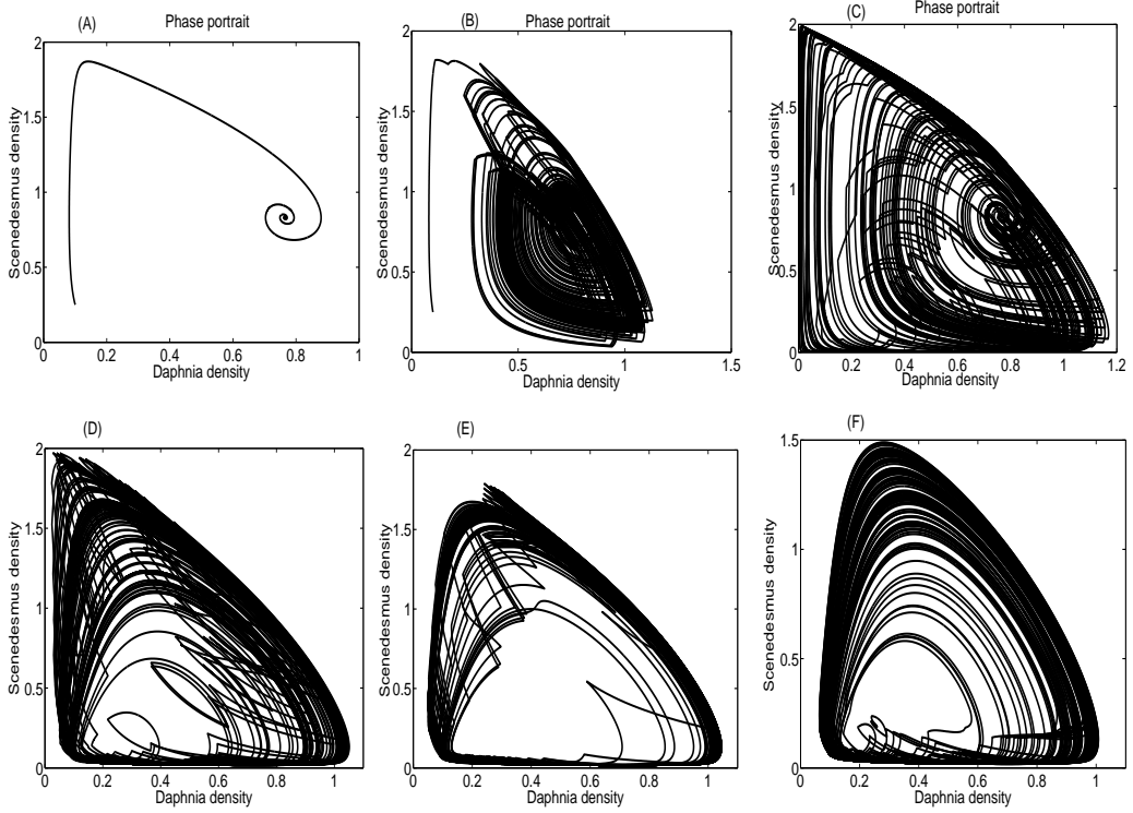
Fig. 5: Daphnia and alga scenedesmus dynamics from model 8 with parameters fixed as in table 1, \sigma = 3 days pulse duration and constant pulse intensity b = 5 \mu\text{gL}^{-1} . (A) is population oscillation dynamics when minimal pulse value Cu_{cst} = 0 . (B) and (C) represents daphnia extinction population from model 8 model 1 respectively, when minimal pulse value Cu_{cst} = 28.3 \mu\text{gL}^{-1} and Cu = 28.3 \mu\text{gL}^{-1} .
