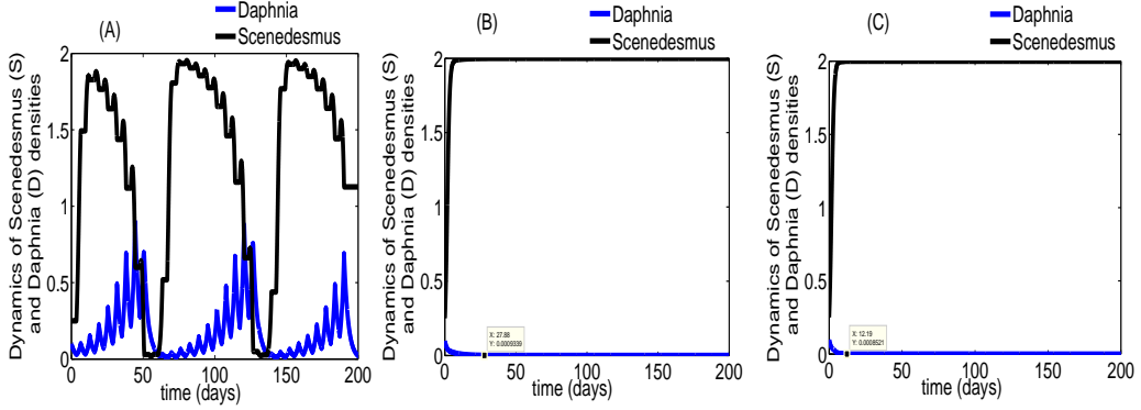
Fig. 4: Daphnia and alga scenedesmus dynamics from model 8 with parameters fixed as in table 1, \sigma = 3 days pulse duration and constant pulse intensity b = 5 \mu gL^{-1} . (A) is population oscillation dynamics when minimal pulse value Cu_{cst} = 0 . (B) and (C) represents daphnia extinction population from model 8 model 1 respectively, when minimal pulse value Cu_{cst} = 28.3 \mu gL^{-1} and Cu = 28.3 \mu gL^{-1} .
