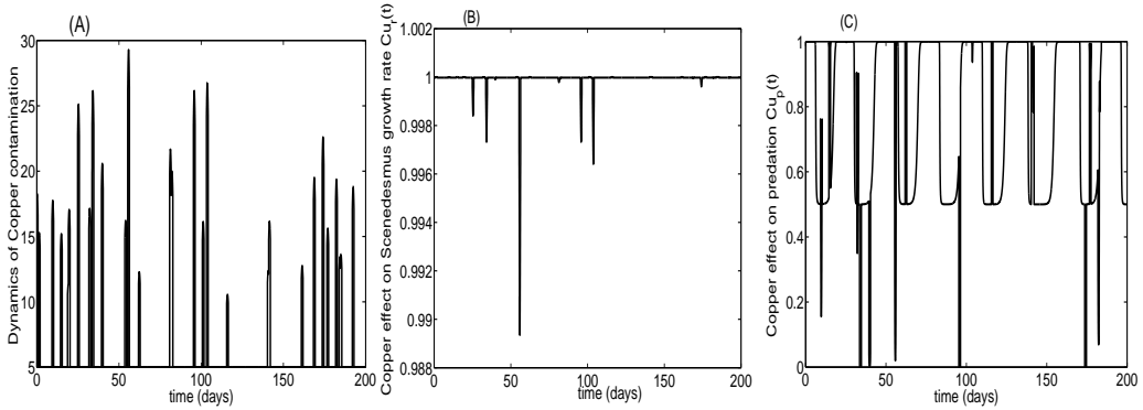
Fig. 2: (A) represents the daily copper concentration Cu(t) from equation 10 with \sigma = 1 days, b follows a \chi^2 distribution with five degree of freedom, Cu_{cst} = 5 \mu g L^{-1} , the number of events N = 30 , time of events t_j follows a uniform distribution in [0, 200 \text{ days}] . (B) and (C) are the correspond measured effects on growth Cu_r(Cu(t)) and predation Cu_p(Cu(t)) .
