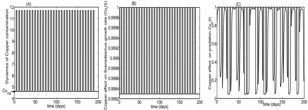
Fig. 1: (A) represents the daily cooper concentration Cu(t) from equation 9 with \sigma = 2 days, b = 7 \mu gL^{-1} , Cu_{cst} = 4.6 \mu gL^{-1} . (B) and (C) are the correspond measured effects on growth Cu_r(Cu(t)) , time of pulse events t_j = 7 \times j days and predation Cu_p(Cu(t)) .
