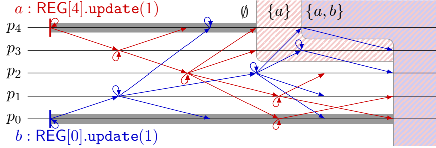
Figure 4: An execution of Algorithm 1. An update is validated by a process when it has received enough messages for this update, and all the other updates it depends of have also been validated.
