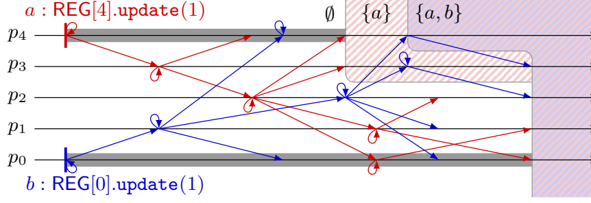
Fig. 4: An execution of Algorithm 1. An update is validated by a process when it has received enough messages for this update, and all the other updates it depends of have also been validated.
