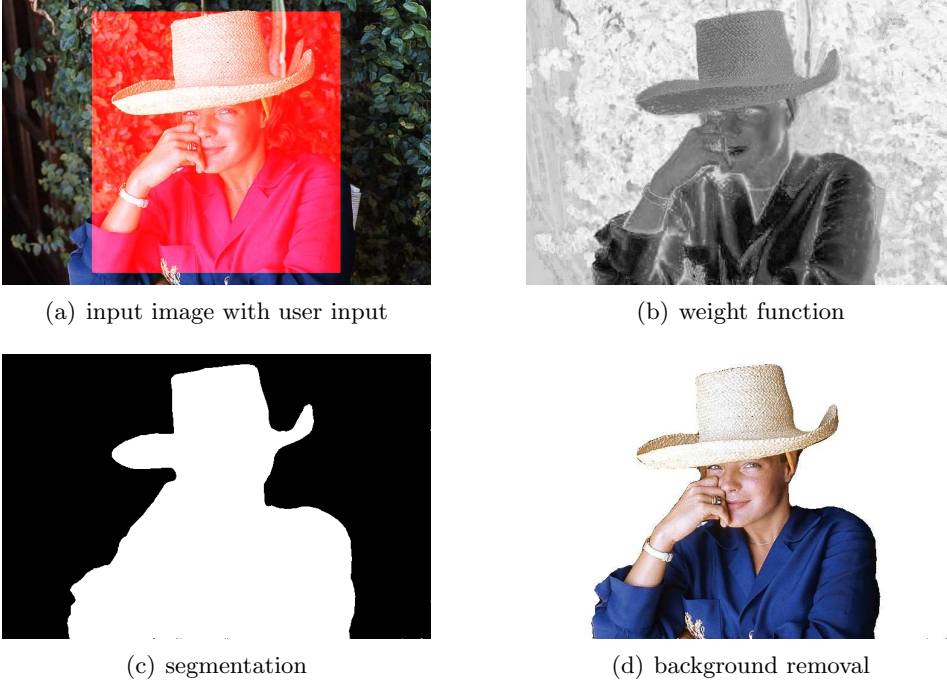
Figure 7.10. Interactive image segmentation using the continuous two-label image segmentation model. (a) Input image overlaid with the initial segmentation provided by the user. (b) The weighting function w , computed using the negative log-ratio of two Gaussian mixture models fitted to the initial segments. (c) Binary solution of the segmentation problem, and (d) the result of performing background removal.
