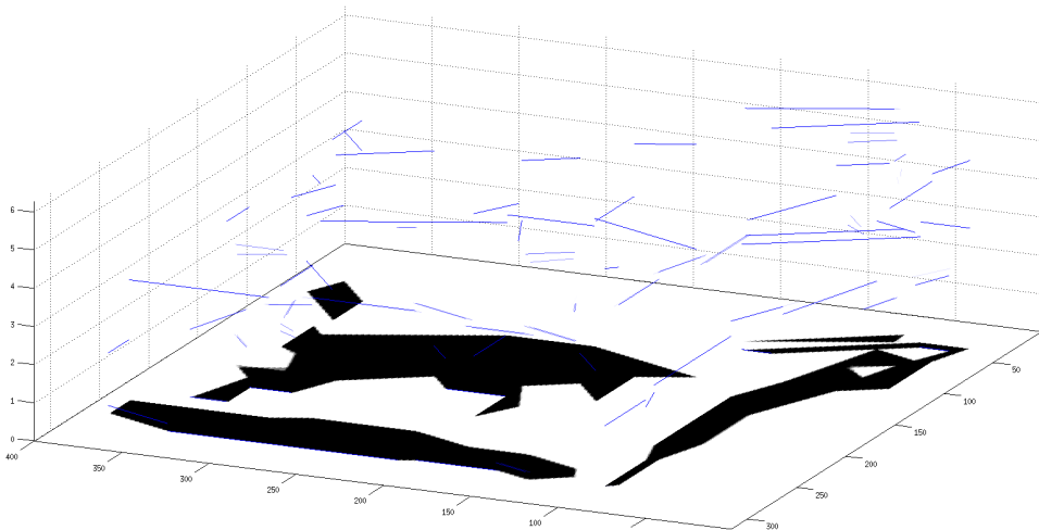
Figure 7.15. Visualization of the measure \mu in the roto-translation space for the image of Figure 7.14(e), obtained using \text{TVX}^0 regularization. Observe that the measure \mu indeed concentrates on thin lines in this space.
