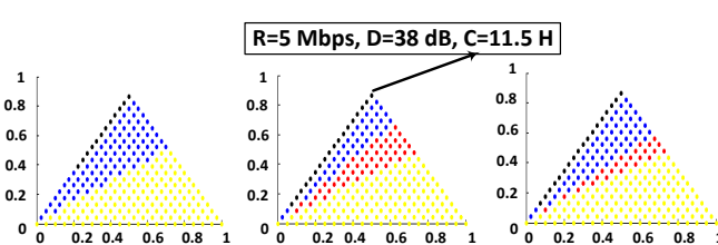
Figure 4: Optimization visualization for three different range of qualities for Sequence#10 "Traffic and building". Left: QP=28, middle: QP=32, and right:QP=36
