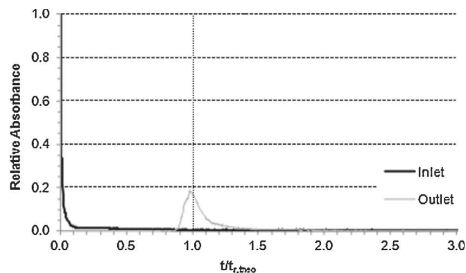
Fig. 5. RTD curve for F_p = 2.7 L h -1 ; Re = 375 .
