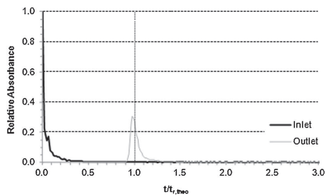
Fig. 6. RTD curve for F_p = 14.8 L h -1 ; Re = 2056 .
