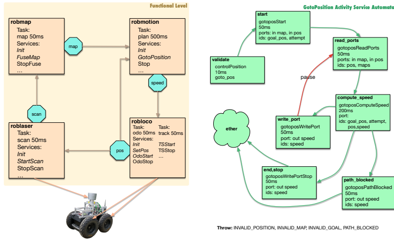
(a) The robot navigation with its four G^{en}M3 modules, their tasks and a partial list of their services (activities are in italic ) (b) The GotoPosition activity automata.
