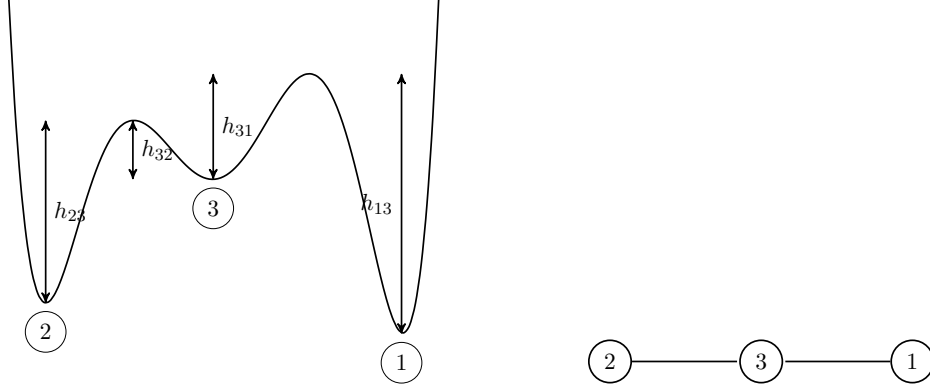
FIGURE 3. Example of a graph associated to a potential.
