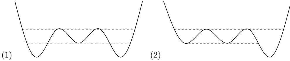
FIGURE 1. Examples of potentials : in (1) we get all eigenvalues, in (2) our theory doesn't work but [12] work.
