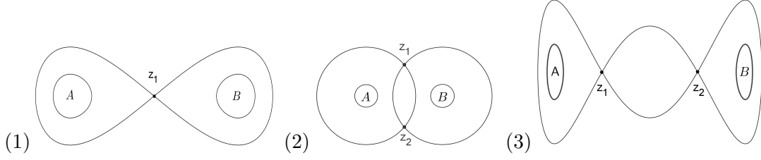
FIGURE 2. Examples of potentials and gates. (1) \mathcal{G}^*(A, B) = \{z_1\} . (2) \mathcal{G}^*(A, B) = \{z_1, z_2\} . (3) \mathcal{G}^*(A, B) = \{z_1\} or \{z_2\} .
