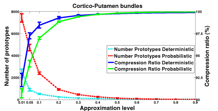
Fig. 7. Evolution of the average number of prototypes and compression ratio at different approximation levels for 5 deterministic and 5 probabilistic cortico-putamen bundles. Bars represent one standard deviation.
