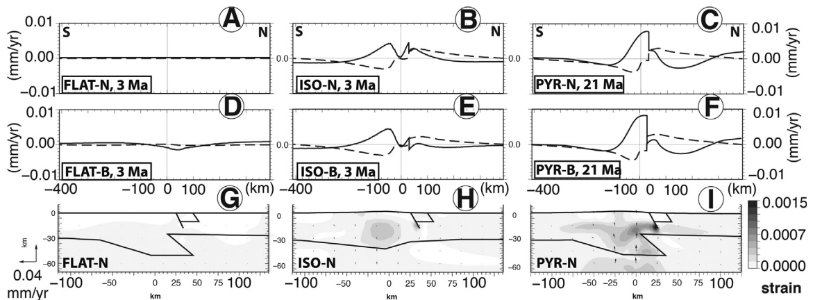
Fig. 4. Strain and surface velocities induced by body forces. This figure can be read as a table; each column corresponds to a geometry, from the left to the right: FLAT, ISO, PYR. The two first rows present final surface velocities profiles: solid and dashed lines correspond respectively to vertical and horizontal velocities. A, B, C. No external solicitation and no dense body (-N). D, E, F. Dense body but no external solicitation (-B). G, H, I. Strain (color palette) and velocity vectors for the experiments with no external solicitation and no dense body.
