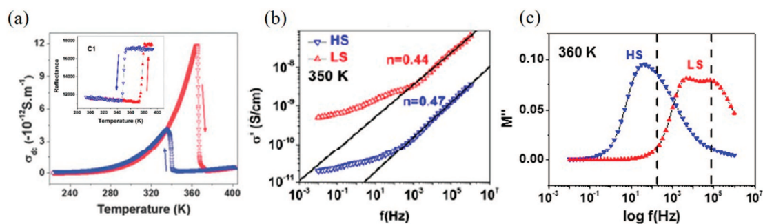
Figure 2. Electrical properties of [\text{Fe}(\text{Htrz})_2(\text{trz})](\text{BF}_4) . (a) Temperature dependence of the dc conductivity in the heating and cooling modes. The inset shows the temperature dependence of the high spin fraction; (b) Spin state dependence of the conductivity spectra at 350 K; (c) Spin-state dependence of the dielectric loss modulus spectra at 360 K. Reprinted from refs. [37] with permission from The Royal Society of Chemistry [38], 2014 WILEY-VCH Verlag GmbH & Co. KGaA © , Weinheim and with permission from [39] Copyright 2015 American Chemical Society.
