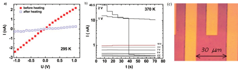
Figure 6. (a) Current-voltage characteristic of the ROM device with [\text{Fe}(\text{HB}(\text{pz})_3)_2] recorded at 295 K before and after heating the device to 408 K; (b) Reading and writing process of the ROM device performed at 370 K; (c) Optical microscopy picture of the micro-electrodes after the deposition of the [\text{Fe}(\text{HB}(\text{pz})_3)_2] film. Reprinted with permission from Ref. [57]. Copyright 2011, AIP Publishing LLC.
