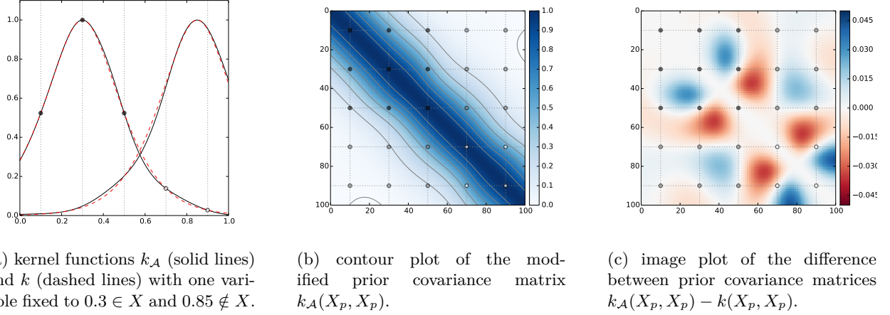
Figure 4: Comparisons of the modified covariance k_A and the initial covariance k . The vector of prediction points X_p corresponds to 100 regularly spaced points spanning [0, 1] . The horizontal and vertical dotted lines correspond to locations of observed points x_i for i \in \{1, \dots, 5\} . The bullets indicate locations where k_A(x_i, x_j) = k(x_i, x_j) .
