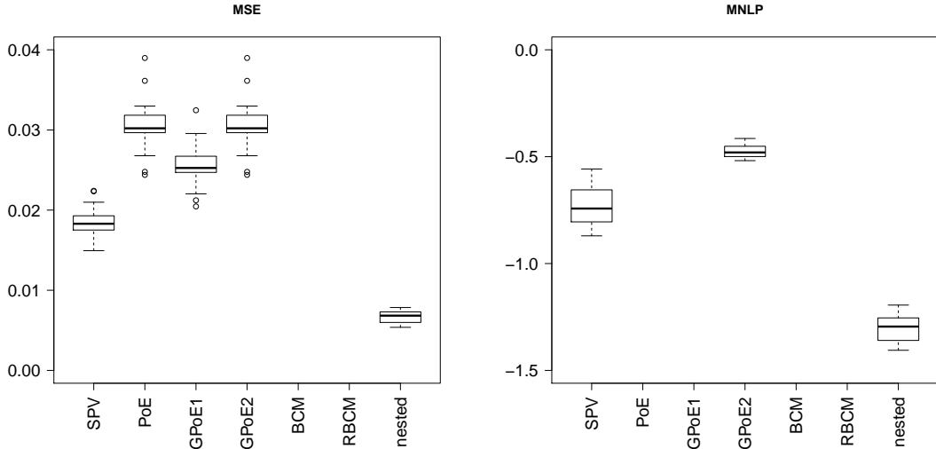
Figure 10: Same settings as in Figure 9 but with p = 90 and where the subsamples are randomly selected. The box plots that are not represented correspond to large MSE or MLNP values. More specifically, the averages (standard deviations) of the 20 MSE values for BCM and RBCM are respectively 0.97 (0.11) and 0.68 (0.071). The averages (standard deviations) of the 20 MNLP values for PoE, GPoE1, BCM and RBCM are respectively 20.6 (2.22), 28.9 (3.29), 441.9 (29.0) and 509 (23.5).
