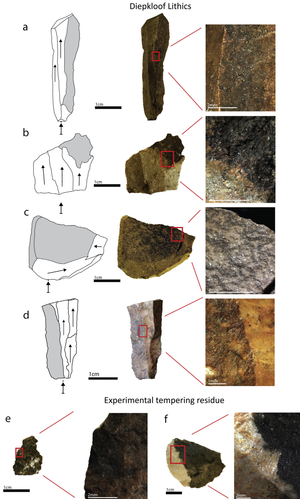
Figure 5. Photographs, technical drawings and Macro-photos of tempering-residue observed on Diepkloof artefacts (a–d) and experimentally heat treated silcrete (e–f). (a) DRSc1, (b) DRSc894, (c) DRSc8, (d) DRSc2676, (e, f) experimentally heat-treated fragments of sample WK-13-08b. Note the black tempering-residue (represented as grey surfaces in the technical drawings) that covers rough pre-heating surfaces. The residue is cut by smooth post-heating fracture negatives of flakes removed after heat treatment (a–d).
