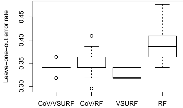
Figure 8: Comparison of leave-one out error rates for proteomic data. CoV/VSURF and CoV/RF correspond to VSURF and random forests (RF) applied on the K^* = 68 synthetic variables given by CoV . VSURF and RF refer to methods applied on the original p = 4786 peptides.
