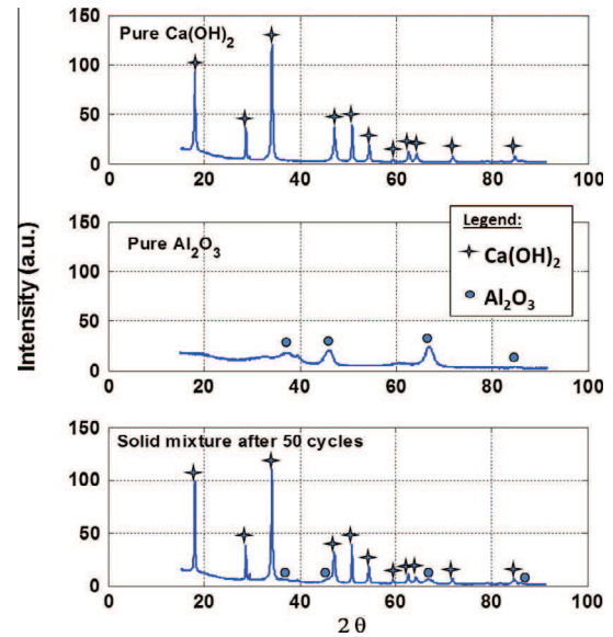
Fig. 14. Diffratograms of pure \text{Ca(OH)}_2 , pure \text{Al}_2\text{O}_3 and 70%w \text{Al}_2\text{O}_3 and 30%w \text{Ca(OH)}_2 mixture after 50 cycles.
