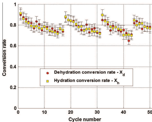
Fig. 13. Conversion rate of both reactions during the cycling study; dehydration: T_w = 480\text{ }^\circ\text{C} - Q_{N_2} = 2\text{ Nm}^3\text{ h}^{-1} - Q_{water} = 0\text{ kg h}^{-1} ; hydration: T_w = 480\text{ }^\circ\text{C} - Q_{N_2} = 2\text{ Nm}^3\text{ h}^{-1} - Q_{water} = 0.49\text{ kg h}^{-1} .
