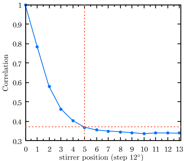
Fig. 4. Correlation coefficient between tuner steps for a frequency around 400 MHz. The value 0.37 corresponds to 5 steps, in perfect agreement with an effective number of uncorrelated stirrer positions N \simeq 6 out of the 30 steps for a complete rotation of the stirrer.
