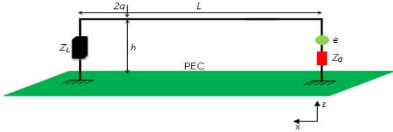
Fig. 4. Validation circuit
