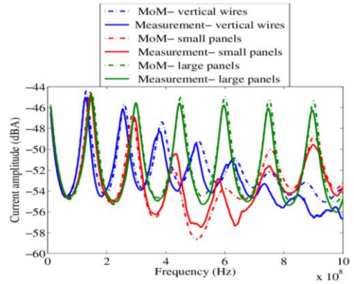
Fig. 6. Current magnitude as a function of the frequency at the end of the transmission line for different terminal configurations
