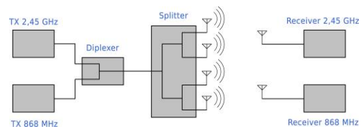
Fig. 2. Global architecture.
