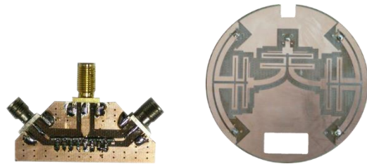
Fig. 6. Photo of the diplexer and splitter prototypes.
