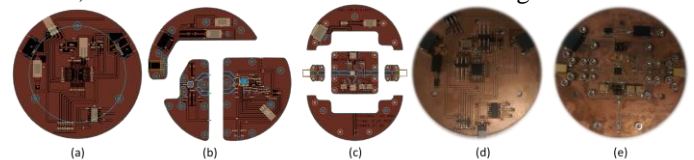
Fig. 3. Designed emitter including, digital stage (a), the modulation stage (b), the power stage (c), pictures of the digital stage (d) and the assembled power stage (e).
