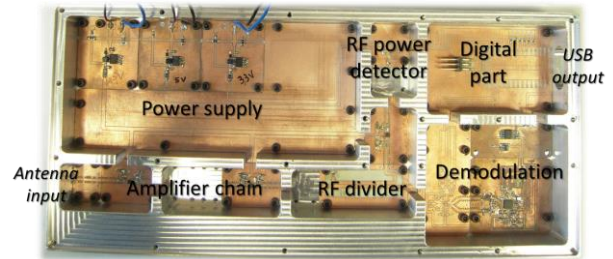
Fig. 7. Picture of the fabricated receiver.
