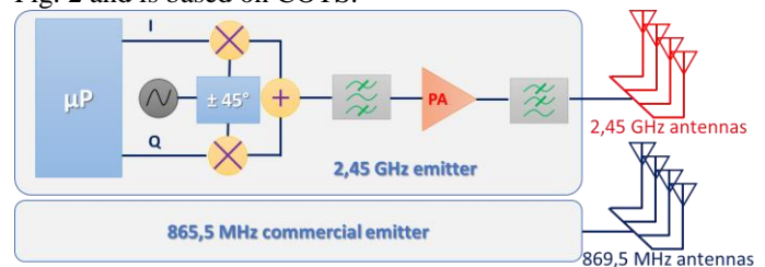
Fig. 2. Dual-band transmitter with 2.45 GHz emitter detailed architecture.
