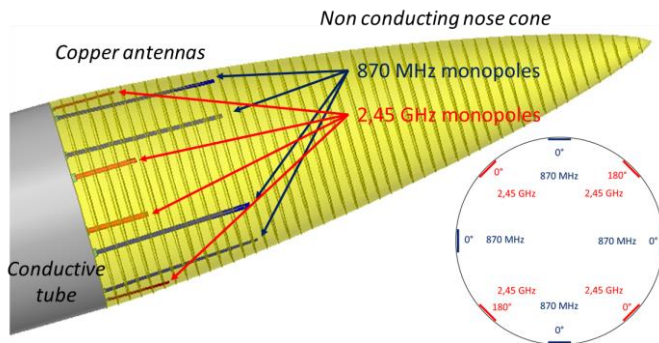
Fig. 4. Architecture of the embedded antenna and phase repartition.
