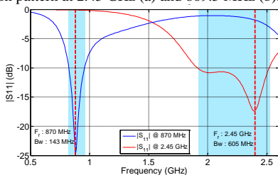
Fig. 6. Impedance matching of the 869.5 MHz and 2.45 MHz antennas.
