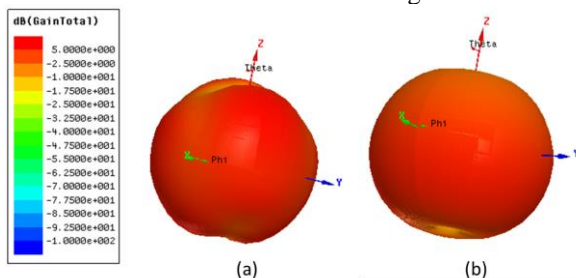
Fig. 5. Radiation pattern at 2.45 GHz (a) and 869.5 MHz (b).
