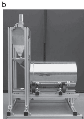
Fig. 8. Solar rotary kiln (a) [19] and (b) [21].
