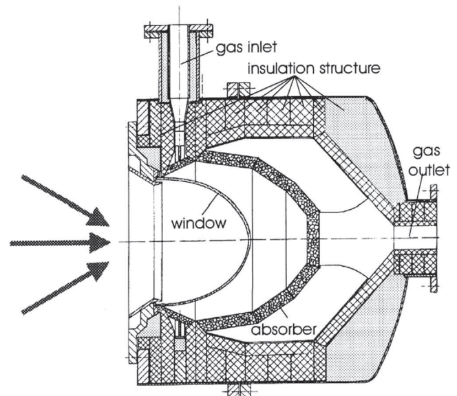
Fig. 19. Schematic of the solar chemical receiver-reactor [64].
