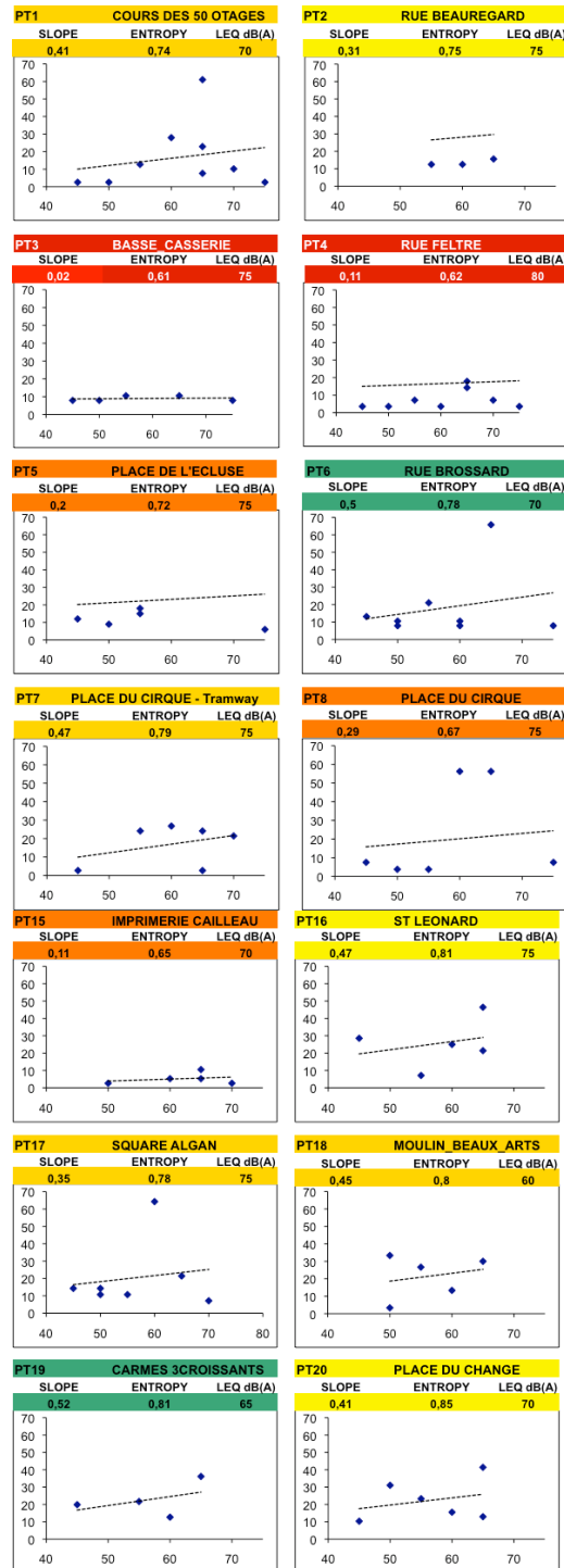
Figure 6. Zipf rank-order laws, entropy values and sound levels for soundwalk points in Nantes city center
