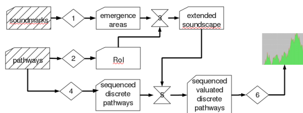
Figure 2. The processing schema we have adopted in the Nantes use case. The sequence is composed of 6 main operations. Input maps are 45 degrees wide hatched, intermediate
