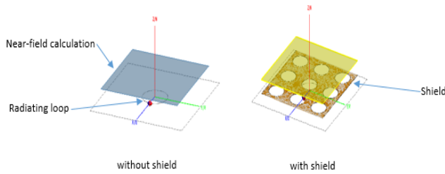
Fig. 2. Near-field configuration
