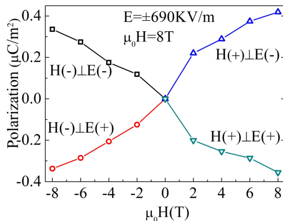
FIG. 10. The induced electric polarization as a function of applied magnetic field with different ME annealing manners.
