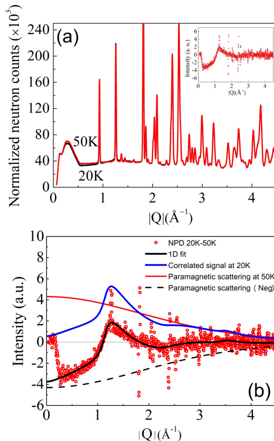
FIG. 7. (a) Comparison between NPD data collected at 20 and 50 K in \text{CaMnGe}_2\text{O}_6 . The inset shows the NPD difference pattern between 20 and 50 K. (b) Diffuse neutron scattering is obtained by subtracting the NPD pattern at 50 K from the pattern at 20 K. The fit corresponds to a 1D AFM correlation model along the zigzag chains (see the text).
