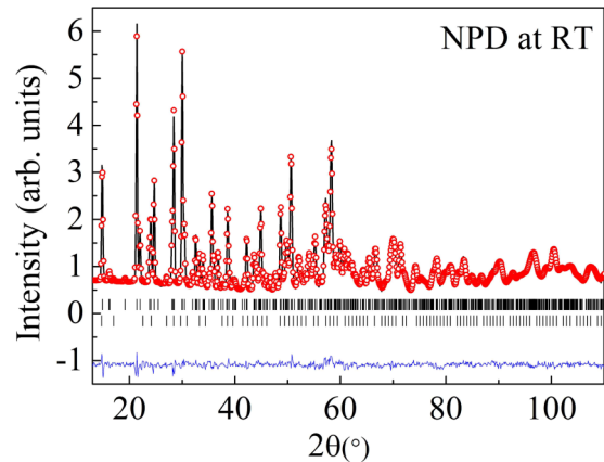
FIG. 1. Rietveld refinement of \text{CaMnGe}_2\text{O}_6 from NPD data taken at room temperature. Observed (open circles), calculated (line), and difference plots (bottom line) are shown. Bragg reflections are denoted by tick marks. The lower set of tick marks belongs to a \text{Ca}_3\text{Mn}_2\text{Ge}_3\text{O}_{12} impurity phase.
