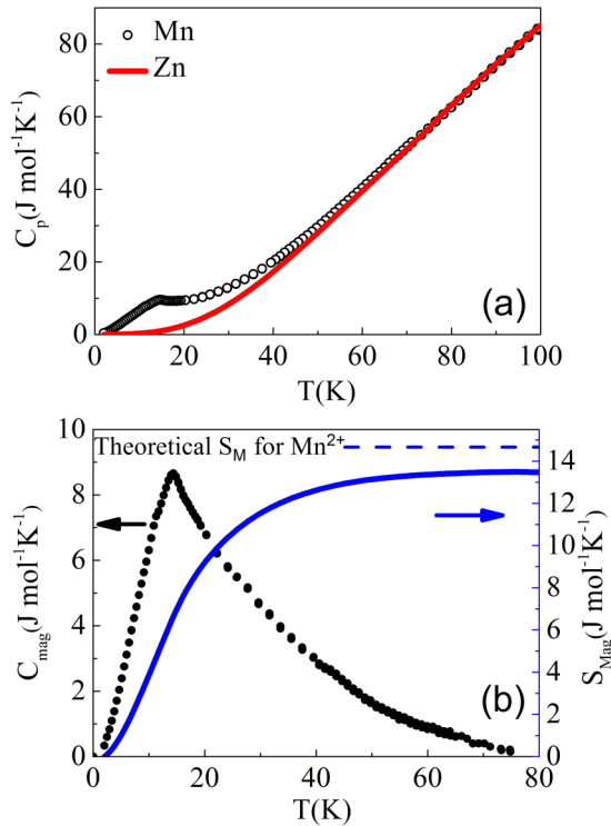
FIG. 4. (a) Specific-heat capacity of \text{CaMnGe}_2\text{O}_6 and \text{CaZnGe}_2\text{O}_6 , which is used as a lattice standard. (b) The magnetic component of the specific-heat capacity of \text{CaMnGe}_2\text{O}_6 ; (blue) the entropy released through magnetic ordering. The blue dashed line represents the theoretical maximum.
