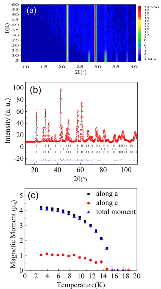
FIG. 5. (a) Plot of neutron powder diffraction scans showing up the magnetic transition at 15 K using a wavelength of 2.52 \text{ \AA} . (b) Observed (open circles) and calculated (line) powder neutron diffraction patterns for \text{CaMnGe}_2\text{O}_6 at 2 K. The lowest tick marks show the magnetic reflections. The nuclear reflections are denoted by upper tick marks. The reflections marked in the middle belong to a \text{Ca}_3\text{Mn}_2\text{Ge}_3\text{O}_{12} impurity phase. The bottom line shows the difference between the observed and calculated diffraction patterns. (c) Evolution of the refined \text{Mn}^{2+} magnetic moment components with temperature.
