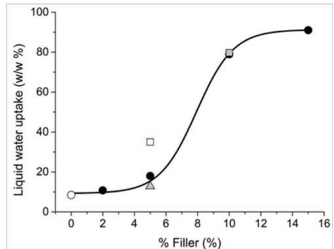
Figure 8. Liquid water uptake as a function of the filler content for neat EVOH (E0, white circle \circ ), and its blends containing 2–15% digestate (D) SLP (black circles \bullet ), 5% compost (CP) SLP (EC5, grey triangle \blacktriangle ), and the blends containing both D and CP SLP in the same sample at total SLP concentration of 5% (ED/C2/3, white square \square ) and 10% (ED/C5/5, grey square \blacksquare ). Samples abbreviations as in Table 2.
