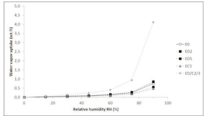
Figure 7. Same as Figure 6 but with a 0–5% zoom along the ordinate-axis (i.e. y \leq 5\% ). Legends: E0 (black solid line, white circles), ED2 (black dotted line, black squares), ED5 (black short-dashed line, black squares), EC5 (dark-grey short-dashed line, dark-grey triangles), ED/C2/3 (light-grey short-dashed line, light-grey diamonds). Samples abbreviations as in Table 2.
