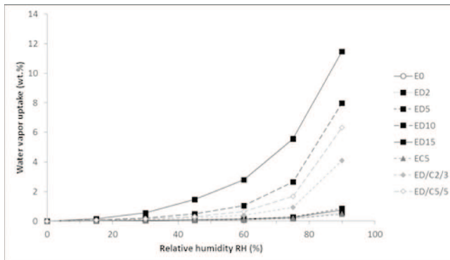
Figure 6. Water vapour sensitivity evaluation by DVS analysis for neat EVOH and blend films. Legends: E0 (black solid line, white circles), ED2 (black dotted line, black squares), ED5 (black short-dashed line, black squares), ED10 (black long-dashed line, black squares), ED15 (black solid line, black squares), EC5 (dark-grey short-dashed line, dark-grey triangles), ED/C2/3 (light-grey short-dashed line, light-grey diamonds), ED/C5/5 (light-grey long-dashed line, white diamonds). Samples abbreviations as in Table 2.
