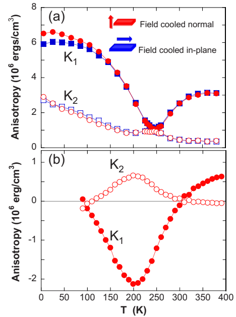
FIG. 3. (Color online) First order ( K_1 ) and second order ( K_2 ) anisotropies fitted from the torque data for sample 1 (a) and sample 2 (b). For sample 1 we include data for both in-plane (squares) and perpendicular (circles) field cooling. For sample 2 the torque curves below 80 K exhibit large hysteresis and become difficult to accurately fit.
