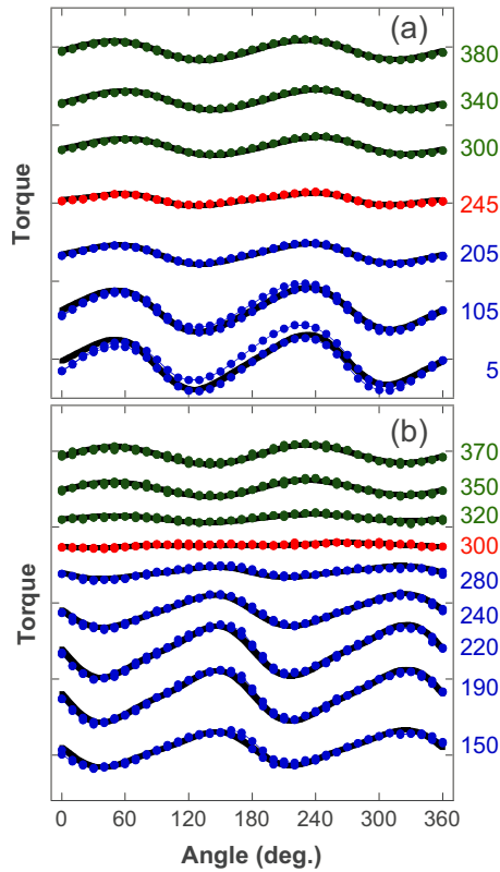
FIG. 2. (Color online) Representative torque curves for sample 1 (a) and sample 2 (b) measured at various temperatures (shown to the right of the graphs). The torque curves have been offset for clarity. For sample 1 there is a minimum in the torque amplitude near \sim 245 K. Below the blocking temperature the torque curves are hysteretic. For sample 2 the torque curves indicate a change in symmetry at 300 K, where the total anisotropy changes from in-plane to perpendicular with increasing temperature. The thick solid lines are fits to the torque curves using Eq. (1) and the results are shown in Fig. 3.
