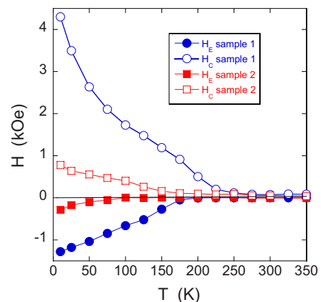
FIG. 1. (Color online) Magnetization results for perpendicular exchange-biased multilayers where sample 1 is CoO(10 Å) × [[Co(4 Å)/Pt(7 Å)] 4 Co(6 Å)CoO(10 Å)] 10 and sample 2 is CoO(10 Å){[Co(8 Å)/Pt(7 Å)] 4 Co(6 Å)CoO(10 Å)] 10 . Plotted are the coercive field H_C and exchange bias H_E for each sample. From these results we estimate the Néel and blocking temperatures to be 250 and 200 K for sample 1 and 200 and 100 K for sample 2, respectively.
