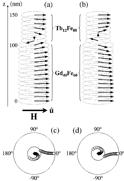
FIG. 2. (a), (b) Schematic representations of the interface domain walls formed in the \text{Gd}_{40}\text{Fe}_{60} (100 nm)/ \text{Tb}_{12}\text{Fe}_{88} (50 nm) bilayer, at room temperature. Shown are the energetically equivalent (a) right handed wall and (b) left handed wall (see Sec. III A for details). (c), (d) Polar plots of the depth dependence of the magnetization azimuthal angle in the interface domain walls sketched in (a), (b). Diamonds and circles correspond to TbFe and GdFe, respectively.
