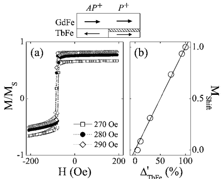
FIG. 3. (a) Examples of minor hysteresis loops measured at 5 K after cooling the sample under H_{cf}=200 Oe in various AP + /P + mixed states corresponding to different values of H'_X , indicated in the legend. (b) Normalized magnetization shift \bar{M}_{Shift} [Eq. (4)], at 5 K, as a function of the fraction of the TbFe layer magnetized in the negative field direction at room temperature, \Delta'_{TbFe} [Eq. (2)]. Errors bars are shorter than the symbol size.
