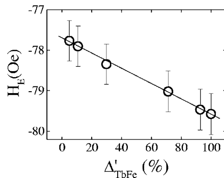
FIG. 4. Exchange-bias field H_E for H_{cf}=200 Oe as a function of the fraction of the TbFe magnetization pointing in the negative field direction \Delta'_{\text{TbFe}} [Eq. (2)]. The line is a guide to the eye.
