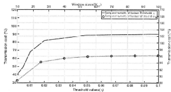
Fig. 4: CH DAWF temporal data relative humidity TX cost metric performances over various thresholds and the various window sizes.
