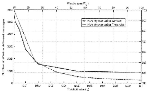
Fig. 2: DAWF different parameter performances with various thresholds Ths over different w_M sizes of temporal data.
