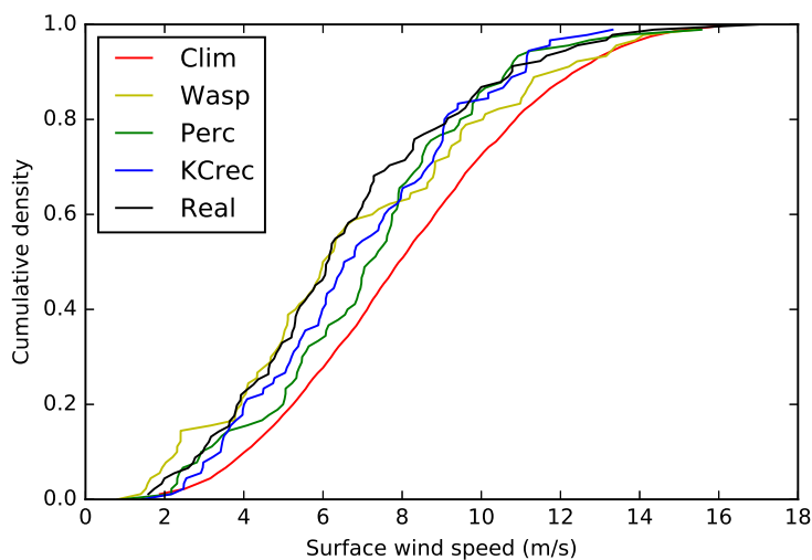
Figure 4: Real, climatological, and reconstructed seasonal CDFs for winter 2012 at 48.5°N 3.0°W
