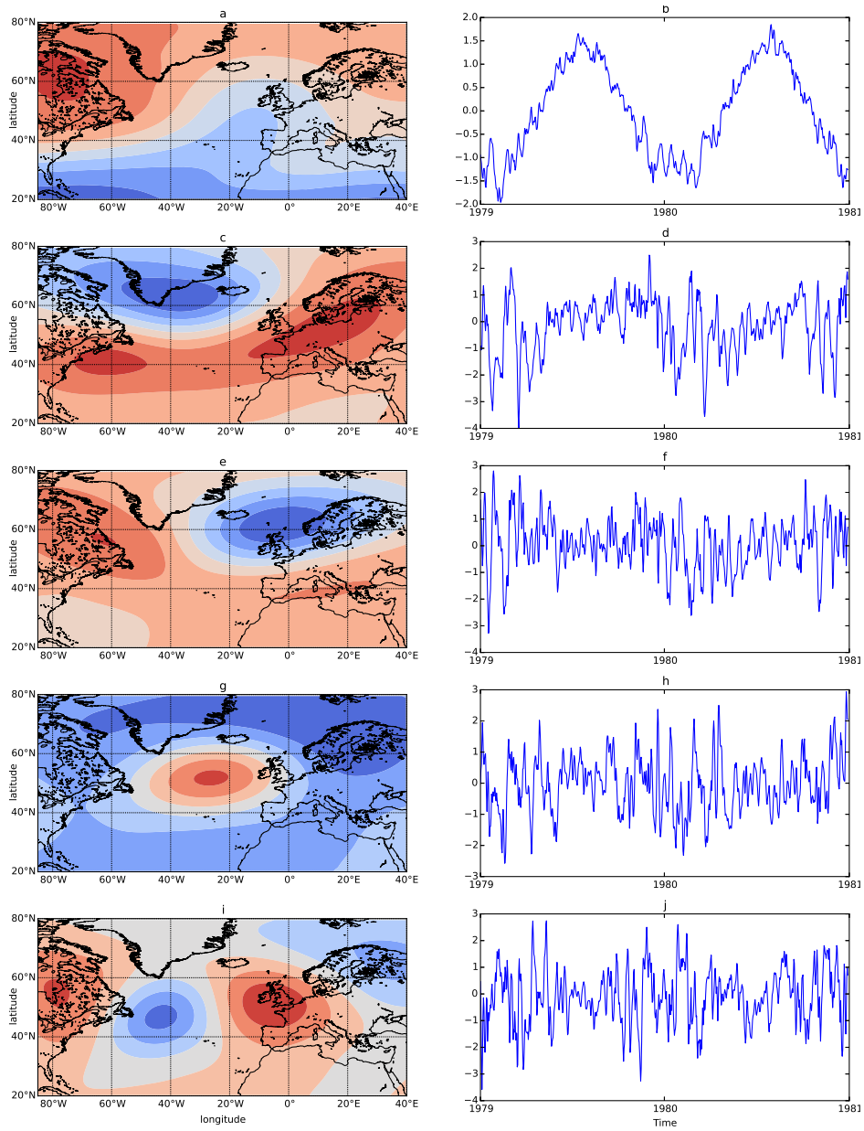
Figure 2: Five first EOFs (left side) and five first PCs (right side) of the PCA performed on the 35 years and on the entire domain of ERAI Z500 dataset
