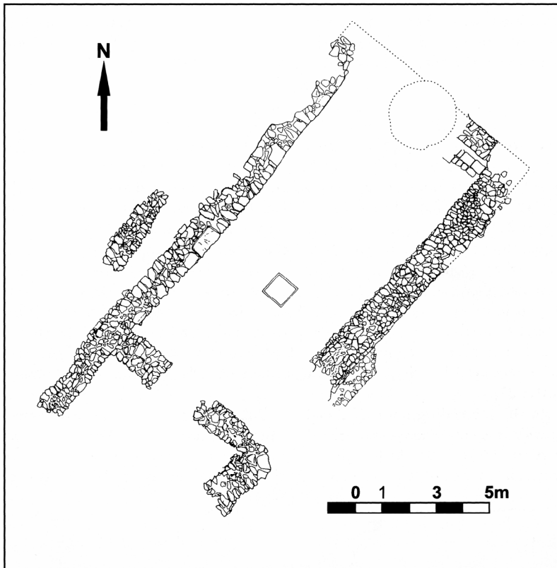
Fig. 15 Plan of Temple L.10 level III-2 at Tell Qara Qûzâq, L. Cooper 2006, 159 fig. 7.9
