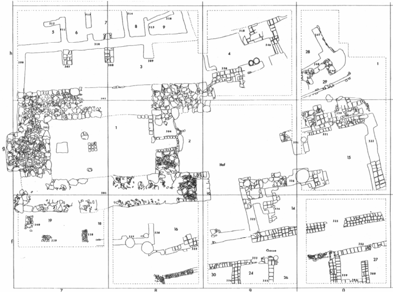
Fig. 16 Plan of Building I (level 3) at Halawa Tell A, W. Orthmann 1989, pl. 10
