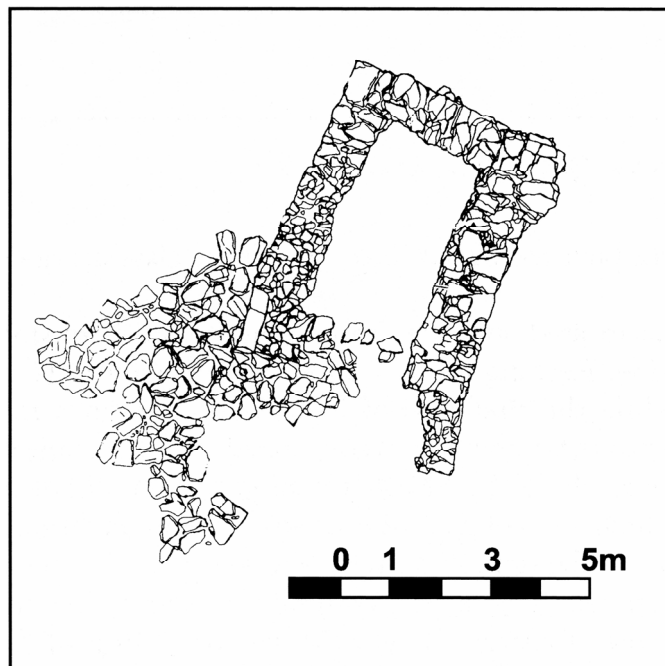
Fig. 14 Plan of Temple L.23 level IV (phase 3) at Tell Qara Qûzâq, G. Del Olmo Lete and J.-L. Montero Fenollos 1998, 297 fig. 2
