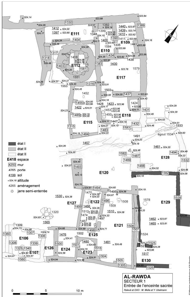
Fig. 3 Schematic plan of the entrance sector in the religious complex at Al-Rawda
