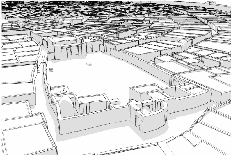
Fig. 6 Restitution of the principal sanctuary of Tell Al-Rawda with the two temples and the sacred enclosure (latest level of occupation) (drawing: Y. Ubelmann). ©Archaeological mission of Al-Rawda
