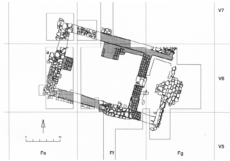
Fig. 13 Plan of Steinbau VI at Tell Chuera, W. Orthmann 2002, fig. 1
