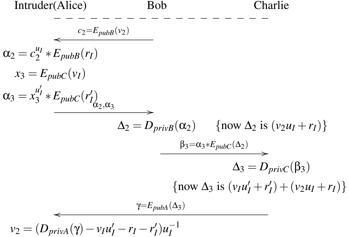
Figure 2: Attack on the secrecy of v_2
