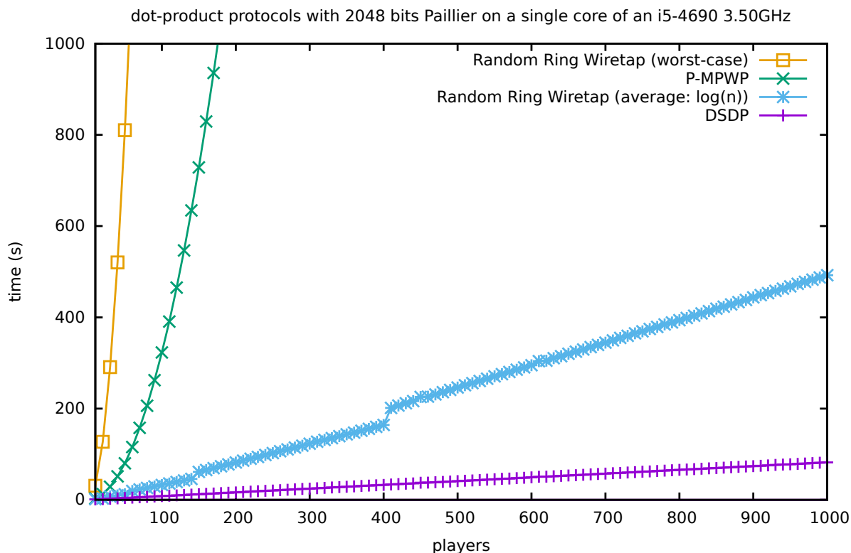
Figure 4: Quadratic and linear protocols timings
