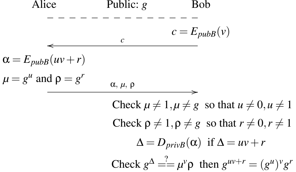
Figure 3: Proof of a non trivial affine transform
