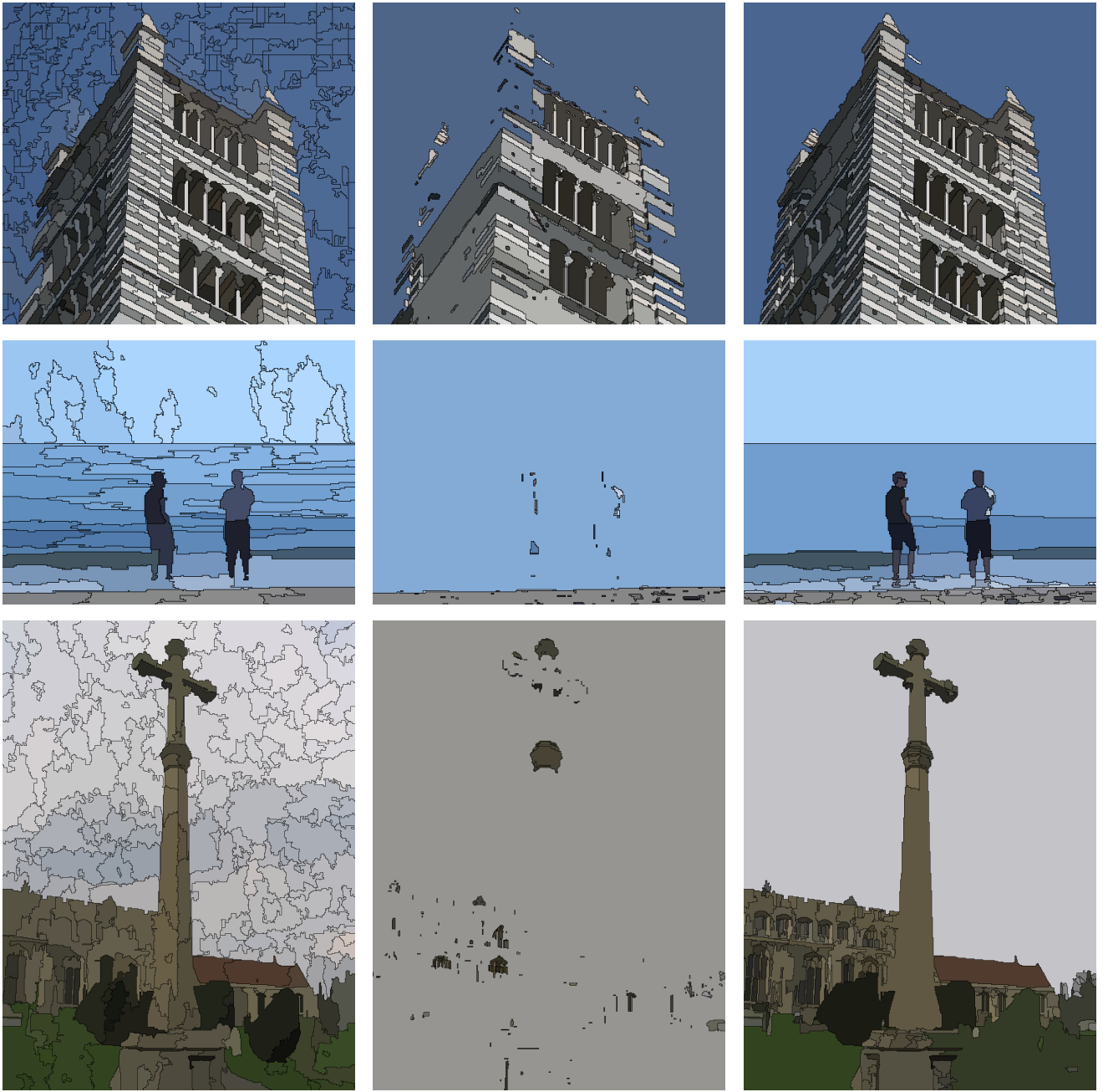
Fig. 9 First and second column: one level of the hierarchies depicted in Figure 7; third column: one level of the hierarchies depicted in Figure 10. First (resp. second, and third) row: the partitions contain 500 (resp. 75, and 250) regions.
