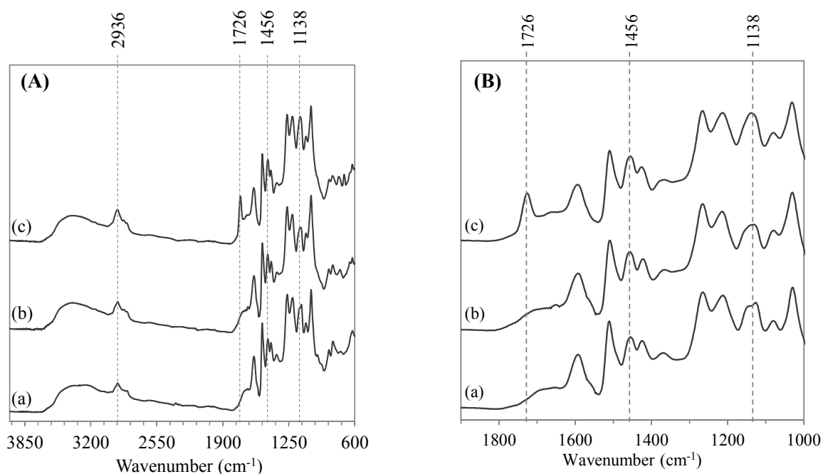
Figure 4. FTIR spectra (A) and their respective zooms of region from 1800 to 1000 \text{cm}^{-1} (B) of original Kraft lignin (a), control Kraft lignin extracted from the [\text{C}_4\text{C}_{1\text{mim}}][\text{OTf}]/[\text{C}_4\text{C}_{1\text{mim}}][\text{PF}_6] binary system without enzyme (b) and lignin oleate extracted from [\text{C}_4\text{C}_{1\text{mim}}][\text{OTf}]/[\text{C}_4\text{C}_{1\text{mim}}][\text{PF}_6] binary system after transesterification catalyzed by the immobilized lipase B from Candida antarctica (c).
