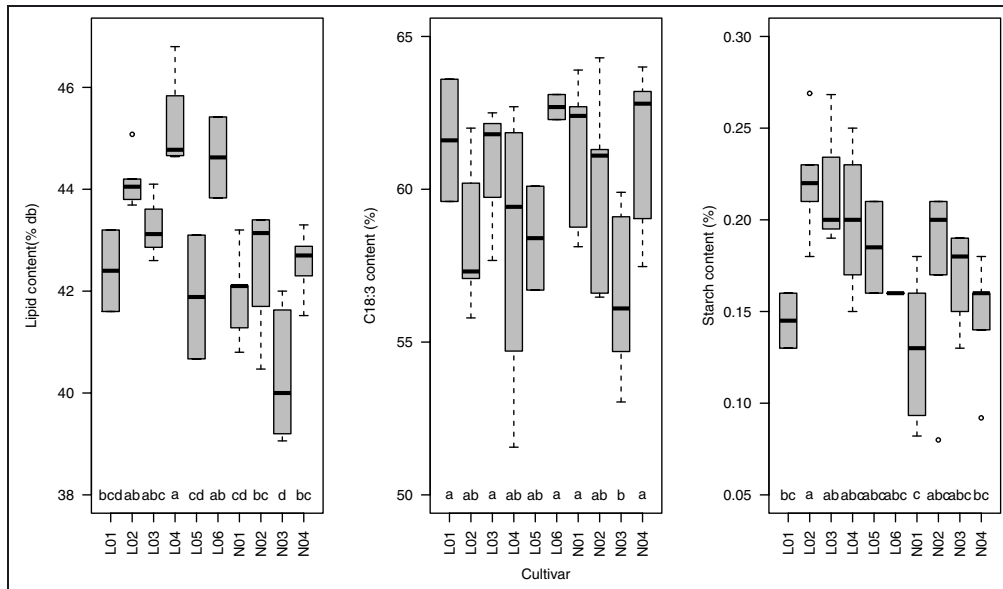
Fig. 2. Boxplots of cultivar significant effect on lipid content, C18:3 content and starch content (means with the same letter are not significantly different according to Tukey HSD test at 95% confidence interval).
