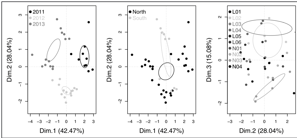
Fig. 5. Individuals representation on PCA dimensions with confidence ellipses. Confidence ellipses are only represented for cultivars L02, L04 and N03.
