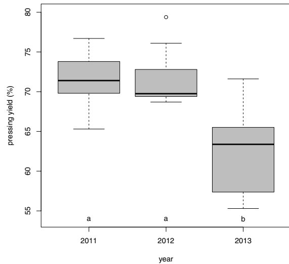
Fig. 6. Boxplots of year significant effect on oil yield.
