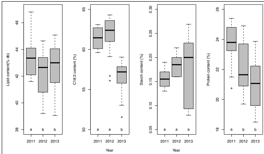
Fig. 1. Boxplots of year significant effect on lipid content, C18:3 content, starch content and protein content (means with the same letter are not significantly different according to Tukey HSD test at 95% confidence interval).
