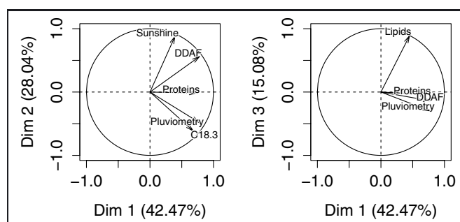
Fig. 4. Variables projection on PCA dimensions 1–2 and 1–3 (only variables with \cos^2 > 0.5 are presented).
