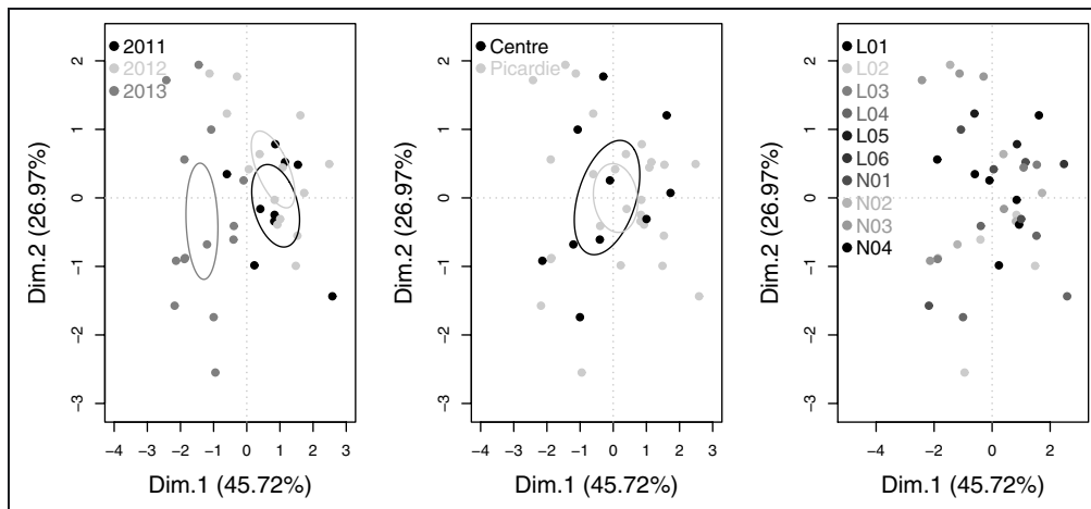
Fig. 8. Individuals representation on PCA dimensions (PCA yield).
