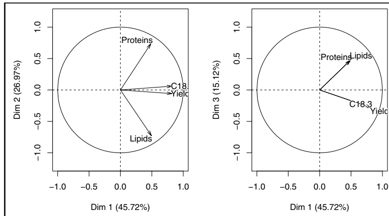
Fig. 7. Variables projection on PCA dimensions 1–2 and 1–3 (PCA yield).
