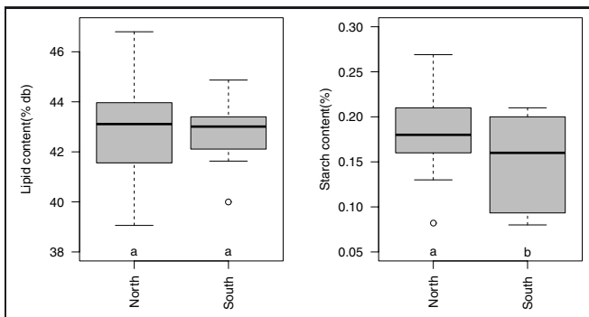
Fig. 3. Boxplots of location significant effect on lipid content, and starch content (means with the same letter are not significantly different according to Tukey HSD test at 95% confidence interval).
