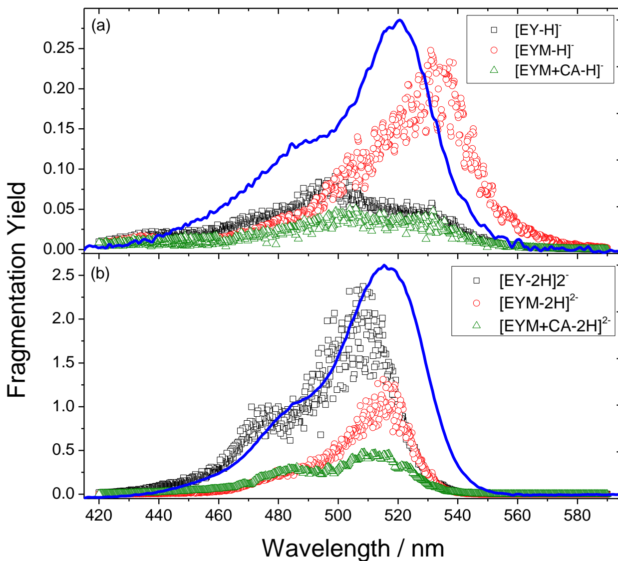
Figure 2. Gas phase action spectra of monoanions (a) and dianions (b) of EY (black squares), EYM (red circles) and EYM+CA, alongside solution phase absorption spectra of EY (solid blue curve) in H_2O at pH 2.53 (a) and 11.87 (b)
