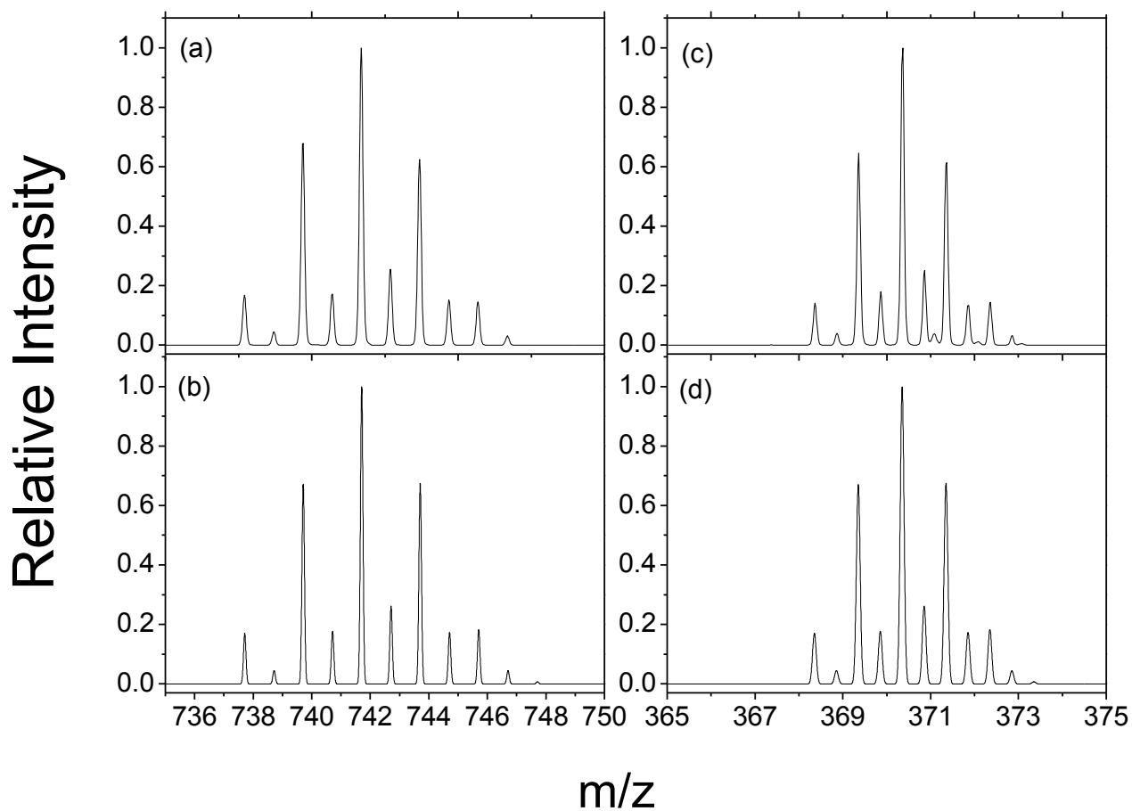
Figure 5. Experimental and theoretical isotopic distribution for mass-selected [\text{EYM-H}]^- (a) and (b) respectively and [\text{EYM-2H}]^{2-} (c) and (d) respectively
