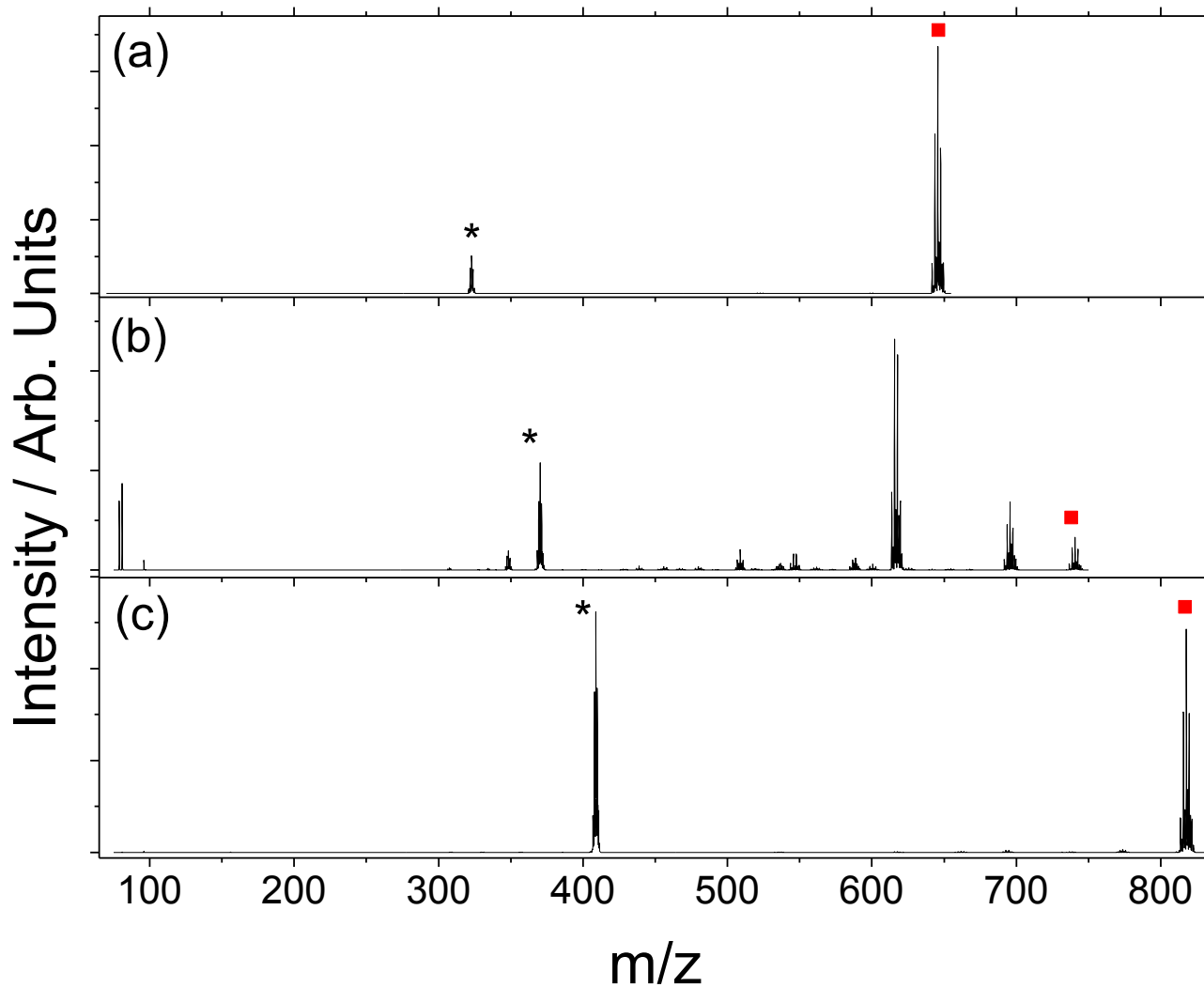
Figure 3. LID mass spectrum of mass selected [EY-2H]^{2-} (a), [EYM-2H]^{2-} (b) and [EYM+CA-2H]^{2-} (c). In each case the asterisk denotes the parent ion, and the red square the photo-detachment channel. All other peaks correspond to fragmentation of the parent ion. The broadening of the peaks is caused by the isotope distribution of Bromine.
