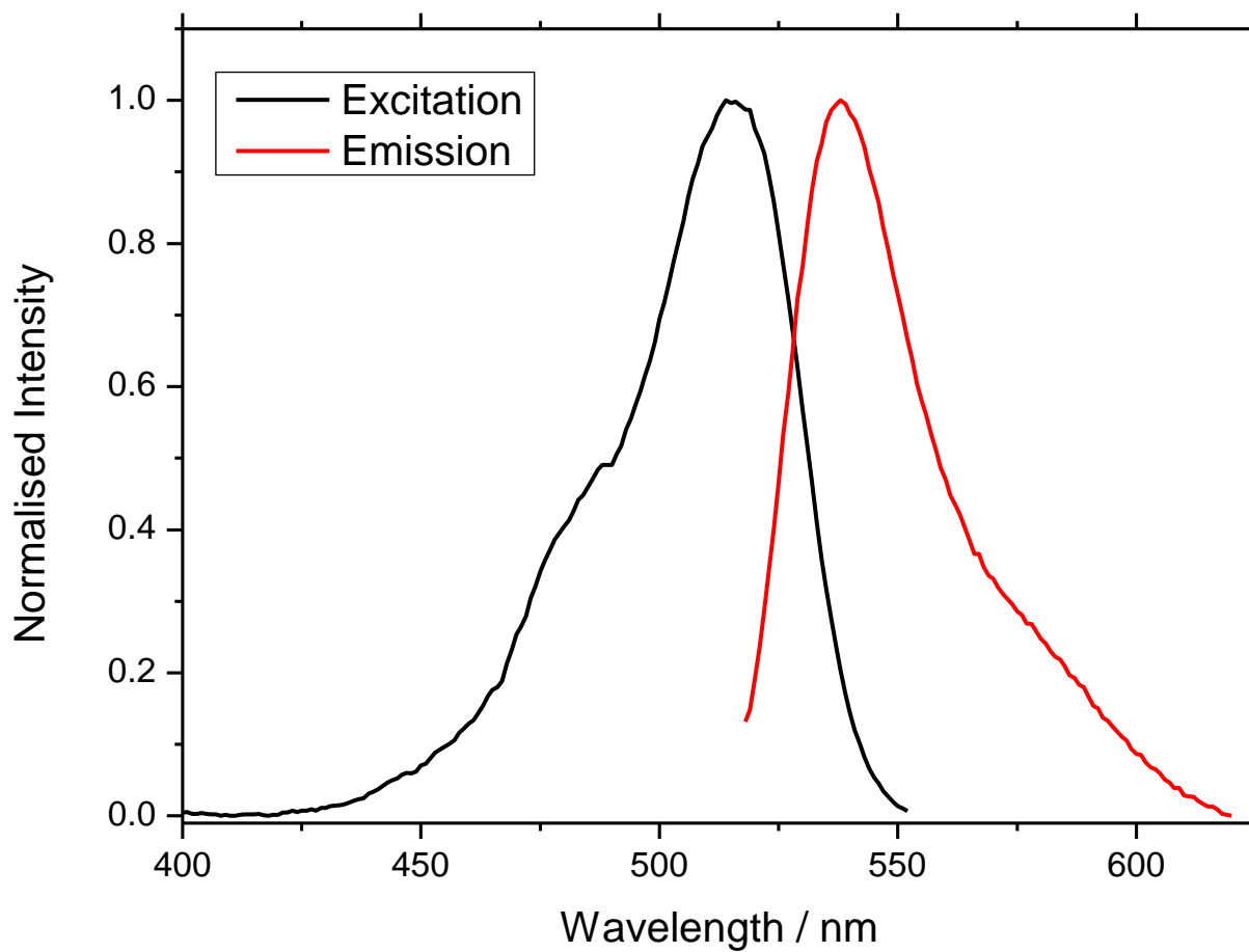
Figure S2. Fluorescence excitation (black) and emission (red) spectra of Eosin Y in H 2 O at pH 11.87.
