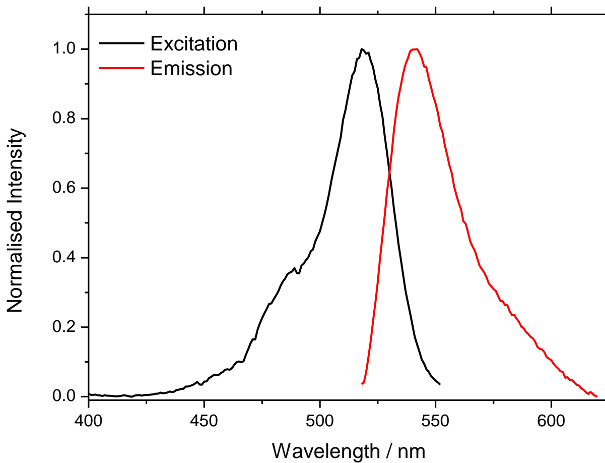
Figure S1. Fluorescence excitation (black) and emission (red) spectra of Eosin Y in H 2 O at pH 2.53.
