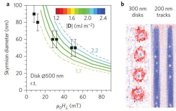
Figure 4 | Evolution of the skyrmion size in patterned nanoscale disks and tracks. a, Magnetic field evolution of the skyrmion size derived from micromagnetic simulations realized for A = 10 \text{ pJ m}^{-1} (lines for different |\mathbf{D}| values) and sizes of the observed skyrmions (squares) for 500-nm-diameter disks. b, R.t. out-of-plane magnetization map of an array of 300-nm-diameter disks with an out-of-plane external field of \mu_0 H_{\perp} = 8 \text{ mT} , and two 200-nm-wide tracks at \mu_0 H_{\perp} \approx 55 \text{ mT} that display several isolated skyrmions.
