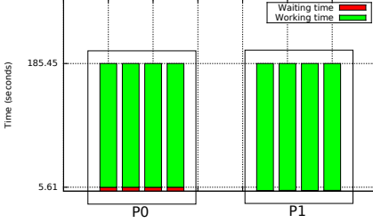
Fig. 14 Load balancing for solving the Quasi group problem (Quasigroup7_10), which is a Constraint Satisfaction Problem using a hybrid parallel programming environment with 2 processors and 4 cores/processor
