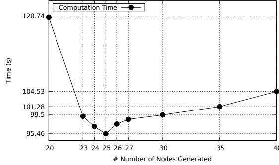
Fig. 2 Variation of computation time for solving the problem of Naval battle (Sb_sb_13_13_5_1) [27] on 12 cores according to the number of sub-trees generated
