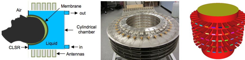
Figure 1: Left: Operating principle of the diagnosis apparatus. Middle: imaging chamber prototype of EMTensor, by courtesy of EMTensor company. Right: the corresponding simulation domain.
