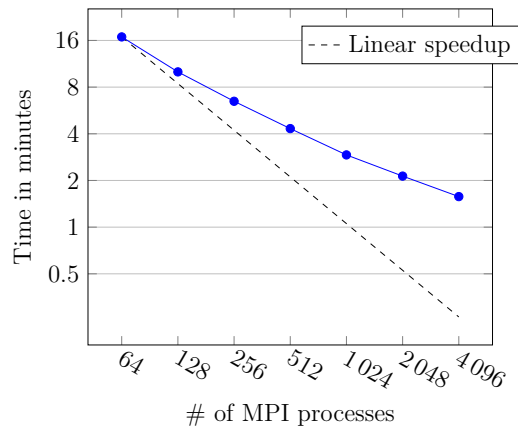
Figure 8: Strong scaling experiment: total time needed to obtain the third reconstructed image shown in Figure 7.
