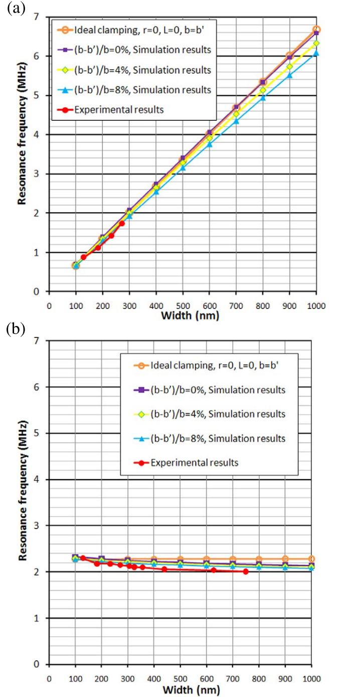
Figure 13. Comparison between experimental and simulation results for the natural frequency evolution as a function of width, with curvature radius at clamping point r = 0.5 \mu\text{m} and with overhanging depth of the cantilever support H = 1.3 \mu\text{m} . Various width variations along the beam's length have been considered ( (b - b')/b = 0\%, 4\% and 8\% ). (a) In-plane mode, (b) out-of-plane mode.
