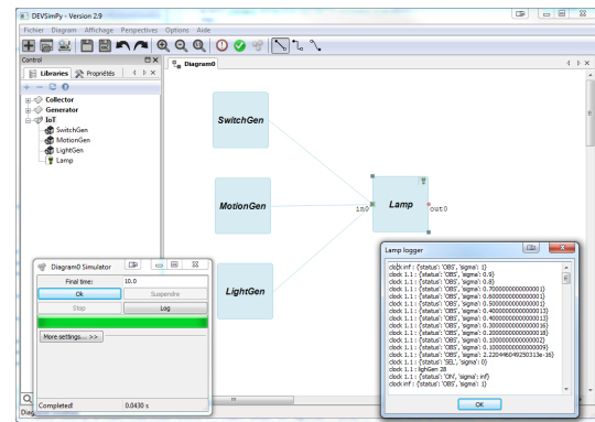
Figure 4: DEVSimPy with simulation dialogue window.
