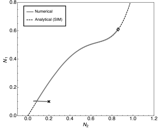
Figure 9: Example 1b. Parameters used: see Eq. (95), a = 0.3 and \mu = 0.7 . Same caption as for Fig. 8.
