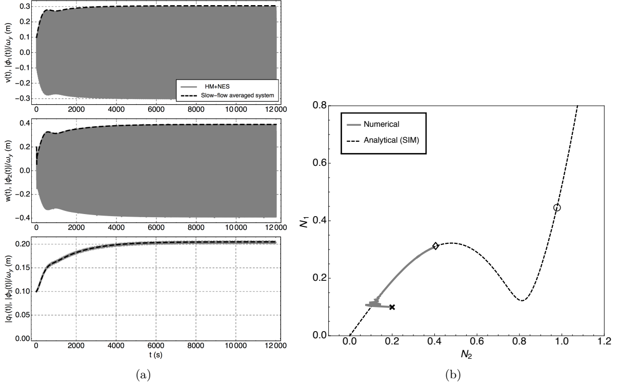
Figure 8: Example 1. Parameters used: see Eq. (95), a = -0.65 and \mu = 0.15 . (a) Comparison between numerical simulation of the HM+NES (24-26) (gray solid line) and the full slow-flow system (47-49) (black dashed line). (b) Comparison between the trajectory of the simulated slow-flow system (47-49) in the plane (N_2, N_1) and the Slow Invariant Manifold (65). "•": position (N_{2,M}, N_{1,M}) , (N_{2,m}, N_{1,m}) , (N_{2,u}, N_{1,M}) and (N_{2,d}, N_{1,m}) , \diamond : stable fixed points, "o": unstable fixed points and \times : initial conditions.
