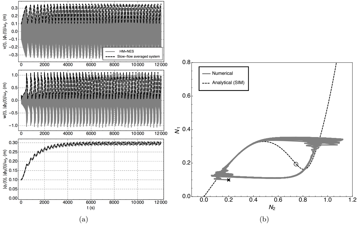
Figure 12: Example 3a. Parameters used: see Eq. (95), a = 0.4 and \mu = 0.2 . Same caption as for Fig. 8.
