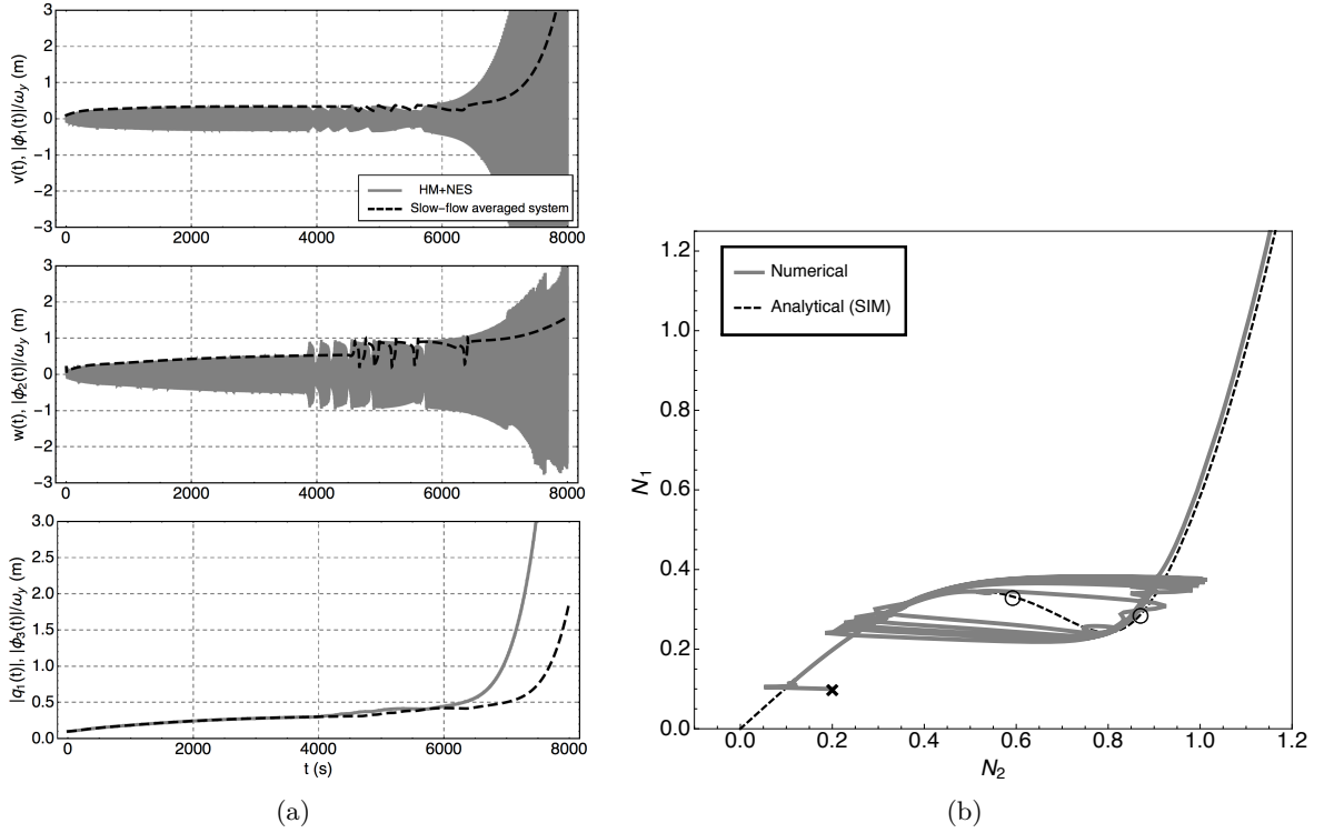
Figure 14: Example 4a. Parameters used: see Eq. (95), a = -0.65 and \mu = 0.3 . Same caption as for Fig. 8.
