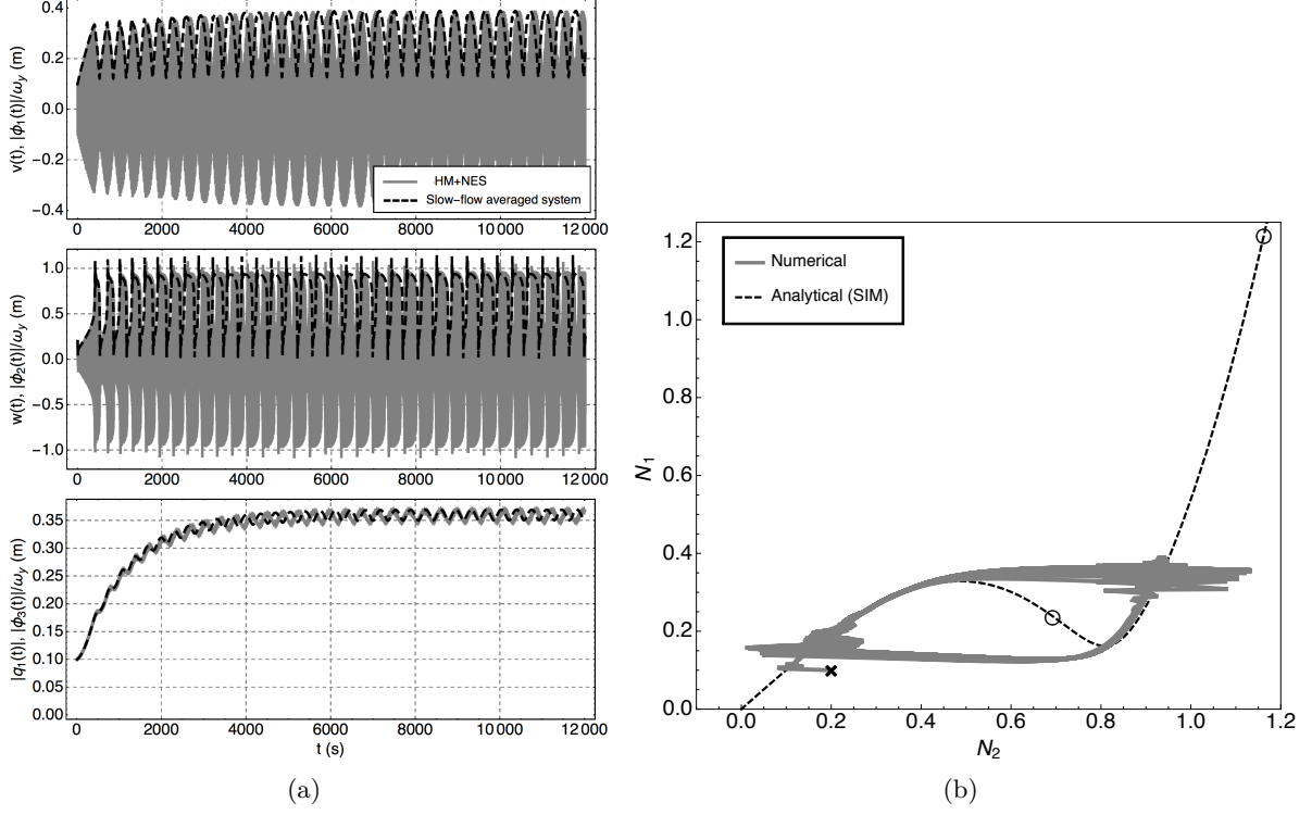
Figure 13: Example 3b. Parameters used: see Eq. (95), a = 0.2 and \mu = -0.2 . Same caption as for Fig. 8.
