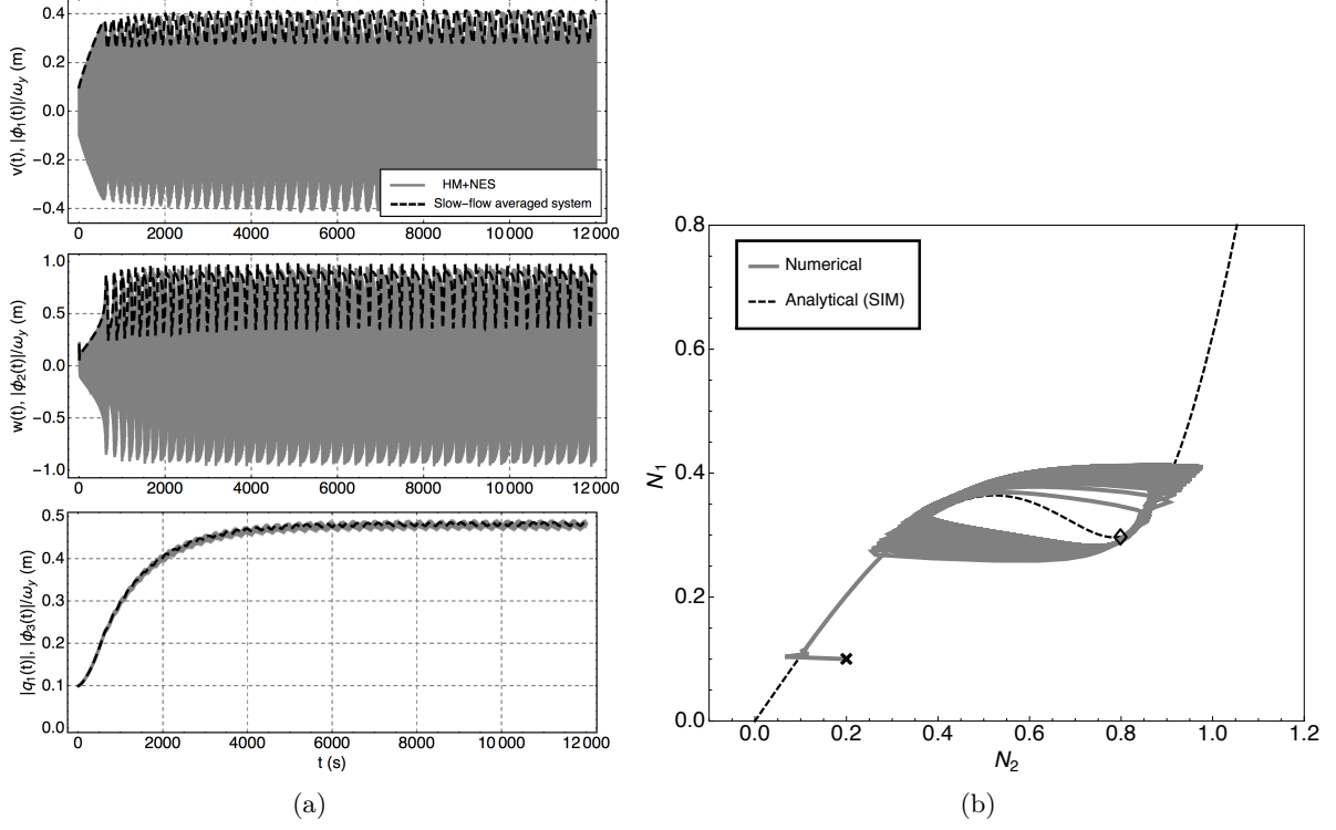
Figure 11: Example 2b. Parameters used: see Eq. (95), a = 0.2 and \mu = 0.37 . Same caption as for Fig. 8.
