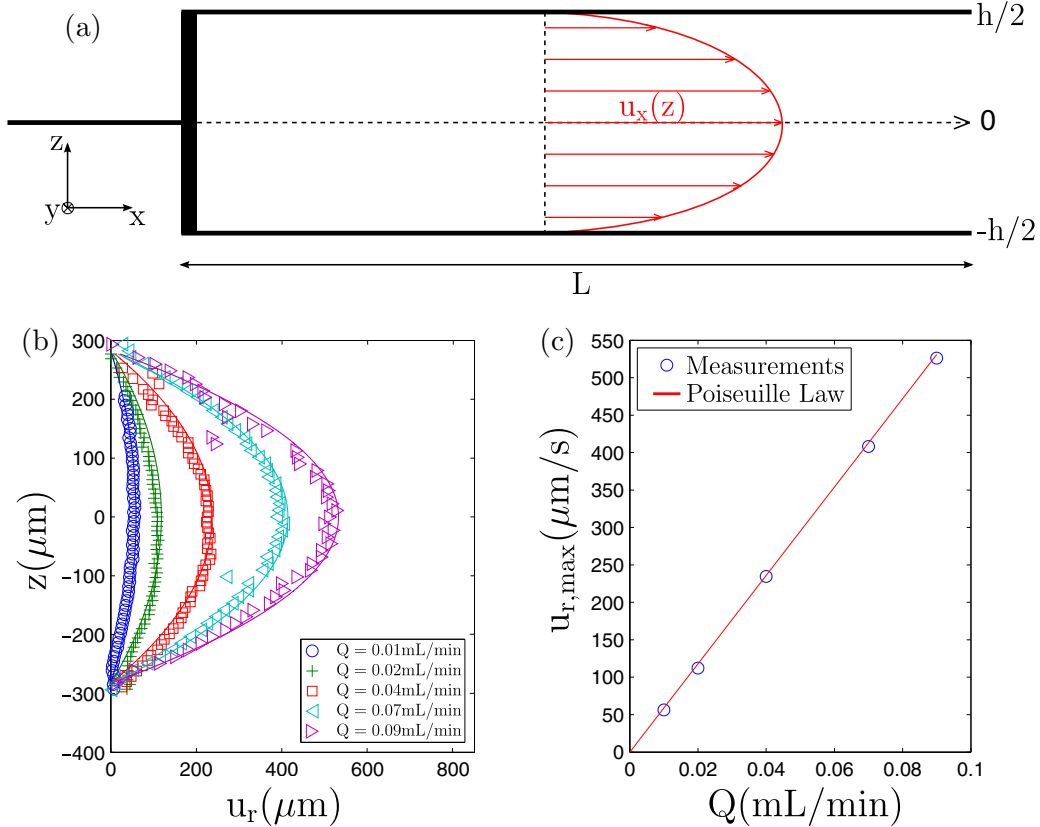
FIG. 9. (a) Schematic of the microchannel (thickness h = 500 \mu\text{m} , width w = 7.5 \text{ mm} , and length L = 10 \text{ cm} ) used for the validation of the PIV. (b) Comparison between velocity measurements (symbols) and the Poiseuille parabolic profile (lines) for several flow rates Q . (c) Variation of the maximum experimental velocity (symbol) with respect to the flow rate compared with the Poiseuille law (line).
