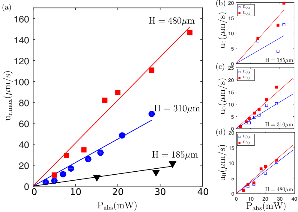
FIG. 5. (a) Comparison between experimental (symbols) and numerical (lines) results for the evolution of the maximum velocity u_{r,\text{max}} with the absorbed power P_{\text{abs}} for each sample height. Variation of the reference velocities u_{0,z} and u_{0,r} determined from u_r(z) and u_r(r) , respectively, for H = 185 \mu\text{m} (b), H = 310 \mu\text{m} (c), and H = 480 \mu\text{m} (d), with respect to the absorbed power (see text).
