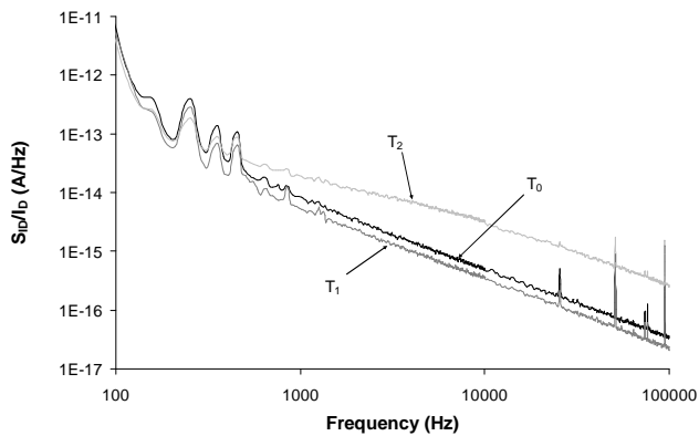
Fig. 5 S_{ID} spectra at T_1 , T_2 and T_3 of non deuterated device
