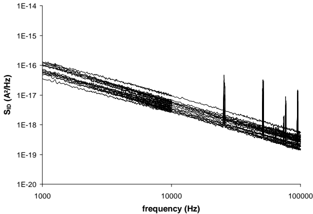
Fig. 3 S_{ID} spectra repartition of batch 1
