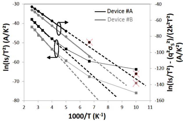
Fig. 7. Conventional and modified Richardson plots of AlGaN/GaN HEMTs. Conventional Richardson plots with the y-axis on the left. Modified Richardson plots by Werner's model with y-axis on the right. Device #A : black lines and dots. Device #B : grey lines and dots.
