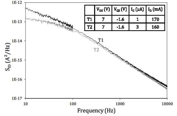
Fig. 7. Drain noise current spectral density of the AlGaIn/GaN HEMTs (T1: non-leaky transistor and T2: leaky transistor) biased at V_{GS}=-1.6V and V_{DS}=7V .
