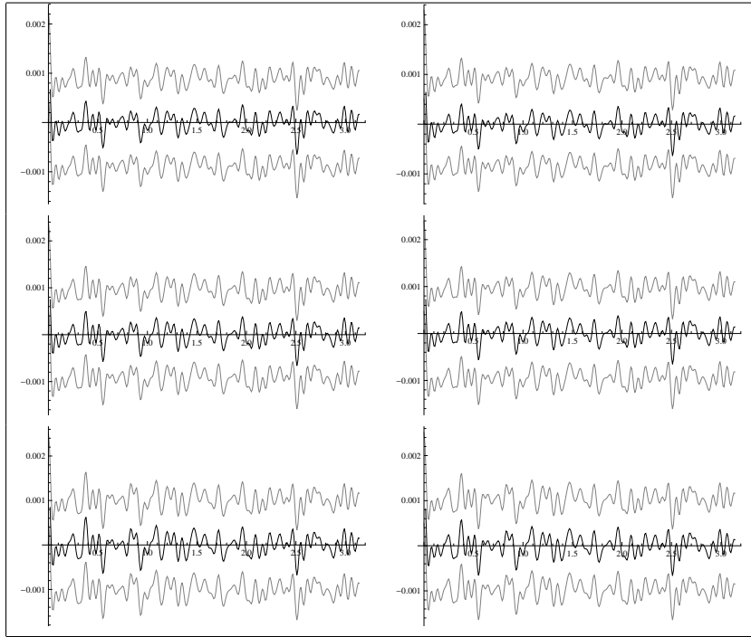
Figure 3: Estimated values of \Re a_X(\lambda, 0) for \lambda \in \{0, 0.01, \dots, 3.14\} and sample size T = 100 , b = 10 (black line) together with the 95% bootstrap simultaneous equal-tailed confidence intervals (gray line) constructed with h = 20T^{-0.35} (left column) and h = 20T^{-0.37} (right column). From top results for d = 0.5, 0.4, 0.2 , respectively.
