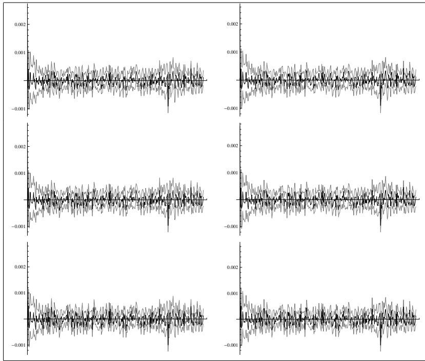
Figure 5: Estimated values of \Re a_X(\lambda, 0) for \lambda \in \{0, 0.01, \dots, 3.14\} and sample size T = 400 , b = 20 (black line) together with the 95% bootstrap pointwise equal-tailed confidence intervals (gray line) constructed with h = 20T^{-0.35} (left column) and h = 20T^{-0.37} (right column). From top results for d = 0.5, 0.4, 0.2 , respectively.
