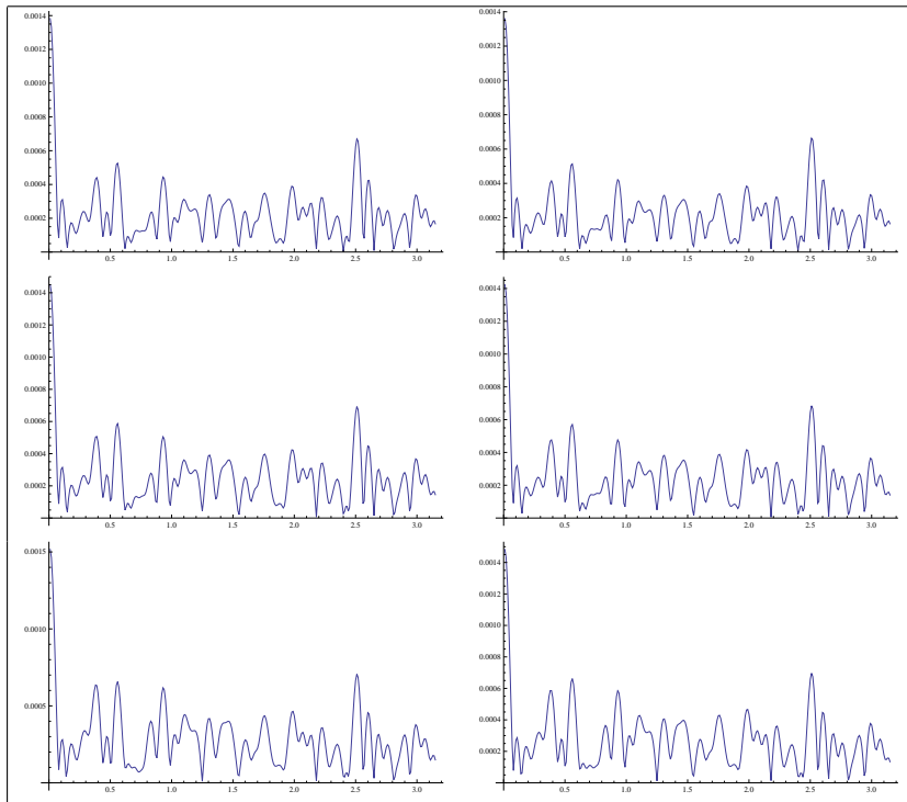
Figure 1: Estimated values of |a_X(\lambda, 0)| for \lambda \in \{0, 0.01, \dots, 3.14\} and sample size T = 100 , b = 10 . Results for h = 20T^{-0.35} and h = 20T^{-0.37} in the left and the right column, respectively. From top results for d = 0.5, 0.4, 0.2 , respectively.
