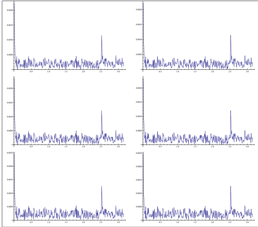
Figure 4: Estimated values of |a_X(\lambda, 0)| for \lambda \in \{0, 0.01, \dots, 3.14\} and sample size T = 400 , b = 20 . Results for h = 20T^{-0.35} (left column) and h = 20T^{-0.37} (right column). From top results for d = 0.5, 0.4, 0.2 , respectively.
