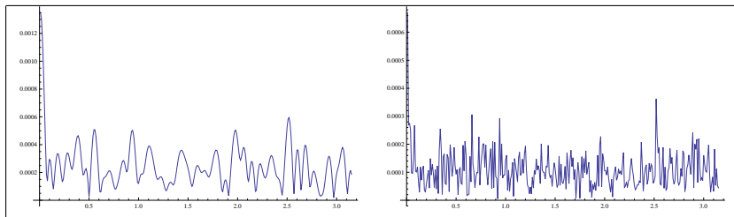
Figure 7: Estimated values of |a_X(\lambda, 1)| for \lambda \in \{0, 0.01, \dots, 3.14\} , sample size T = 100 (left panel) and T = 400 (right panel), b = \lfloor T^{1/2} \rfloor , h = 20T^{-0.37} and d = 0.2 .
