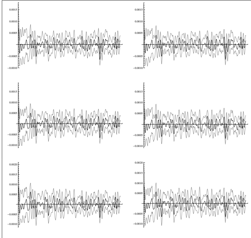
Figure 2: Estimated values of \mathfrak{R}a_X(\lambda, 0) for \lambda \in \{0, 0.01, \dots, 3.14\} and sample size T = 100 , b = 10 (black line) together with the 95% bootstrap pointwise equal-tailed confidence intervals (gray line) constructed with h = 20T^{-0.35} (left column) and h = 20T^{-0.37} (right column). From top results for d = 0.5, 0.4, 0.2 , respectively.
