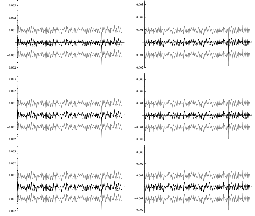
Figure 6: Estimated values of \Re a_X(\lambda, 0) for \lambda \in \{0, 0.01, \dots, 3.14\} and sample size T = 400 , b = 20 (black line) together with the 95% bootstrap simultaneous equal-tailed confidence intervals (gray line) constructed with h = 20T^{-0.35} (left column) and h = 20T^{-0.37} (right column). From top results for d = 0.5, 0.4, 0.2 , respectively.
